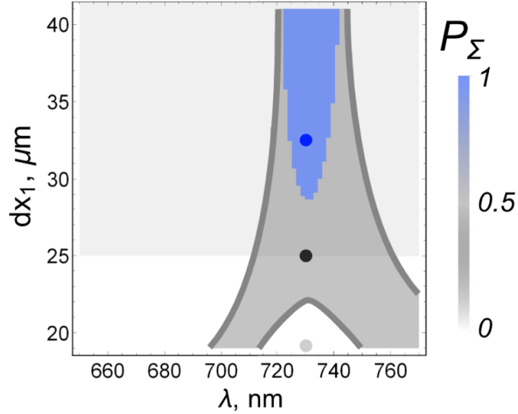
Figure 7.5: Topological phase diagram.
