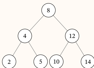
Prima: Delete(T, 8)
