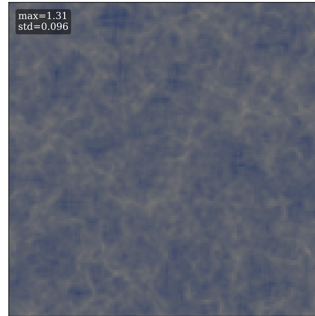
kcorr royal-energy-58
