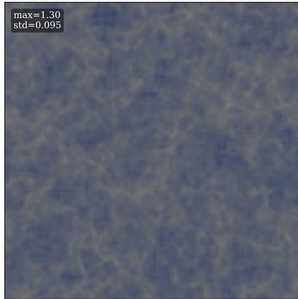
LR (baseline)
