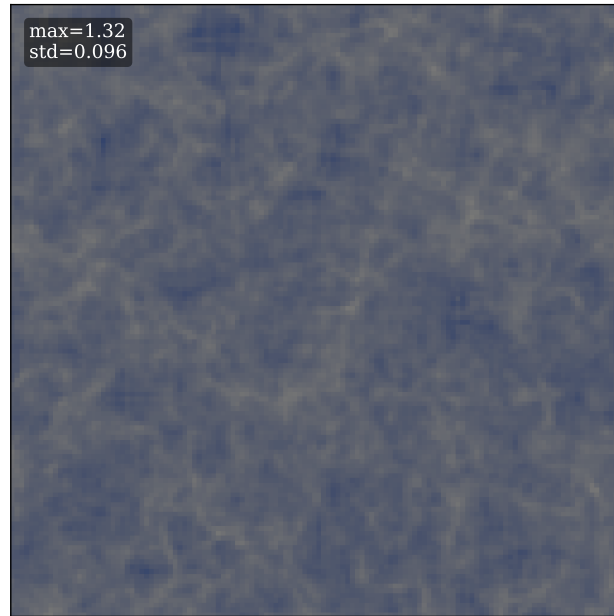
cnn electric-dream
