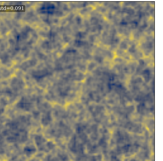
kcorr royal-energy-58
