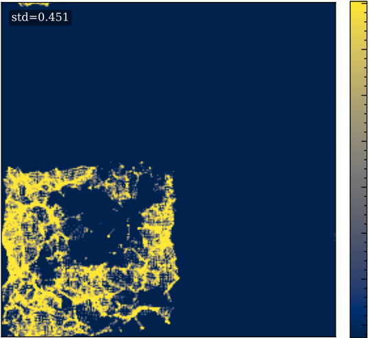
HR (target)
