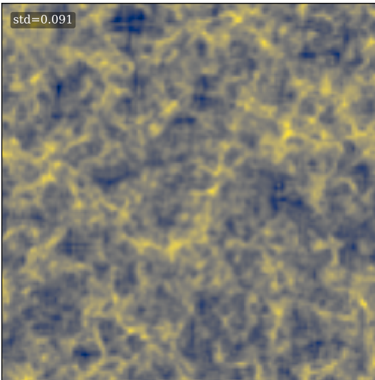
cnn electric-dream
