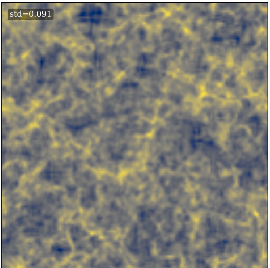
cnn glorious-wood-80
