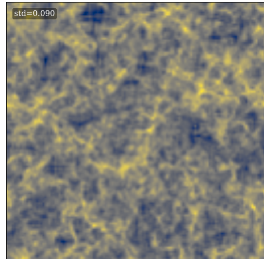
LR (baseline)
