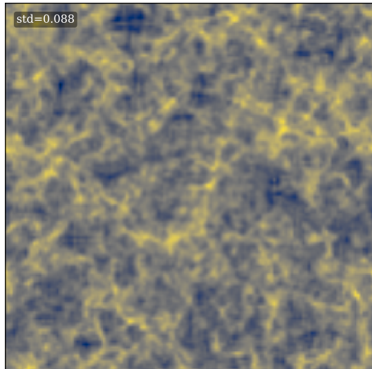
kcorr gallant-lion-73
