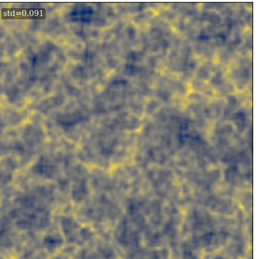
cnn revived-grass-60
