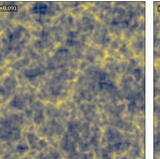
cnn young-field-77
