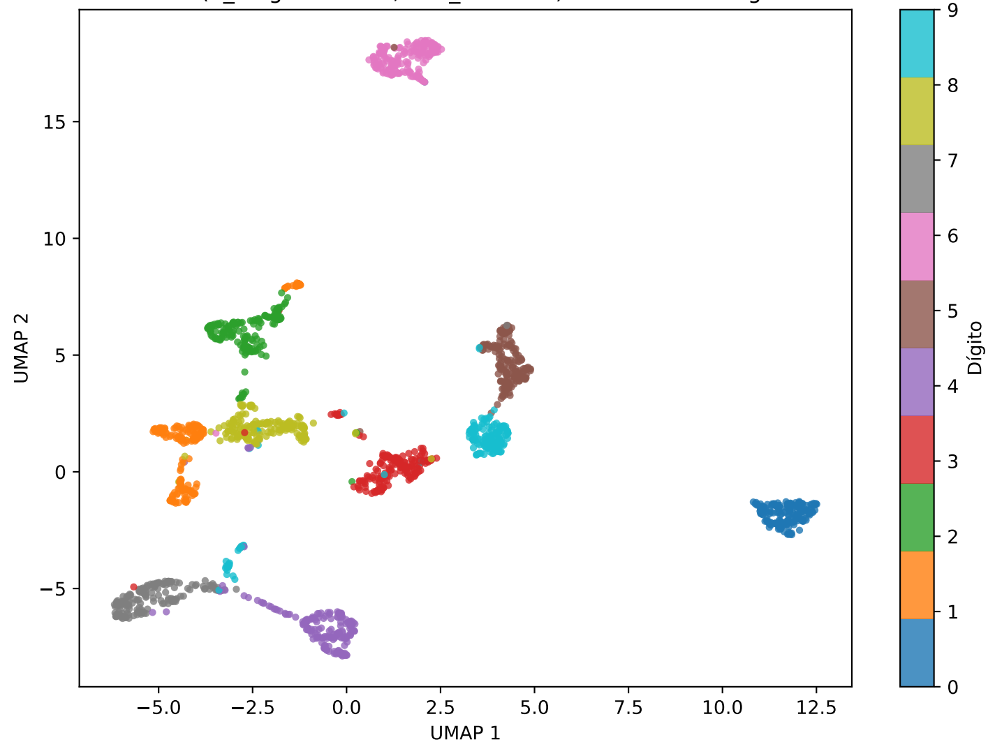
UMAP (n_neighbors=15, min_dist=0.1) — dataset de dígitos
