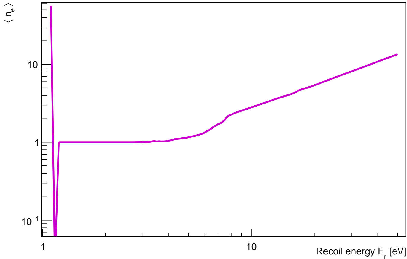
Mean electron yield \langle n_e \rangle vs E_r
