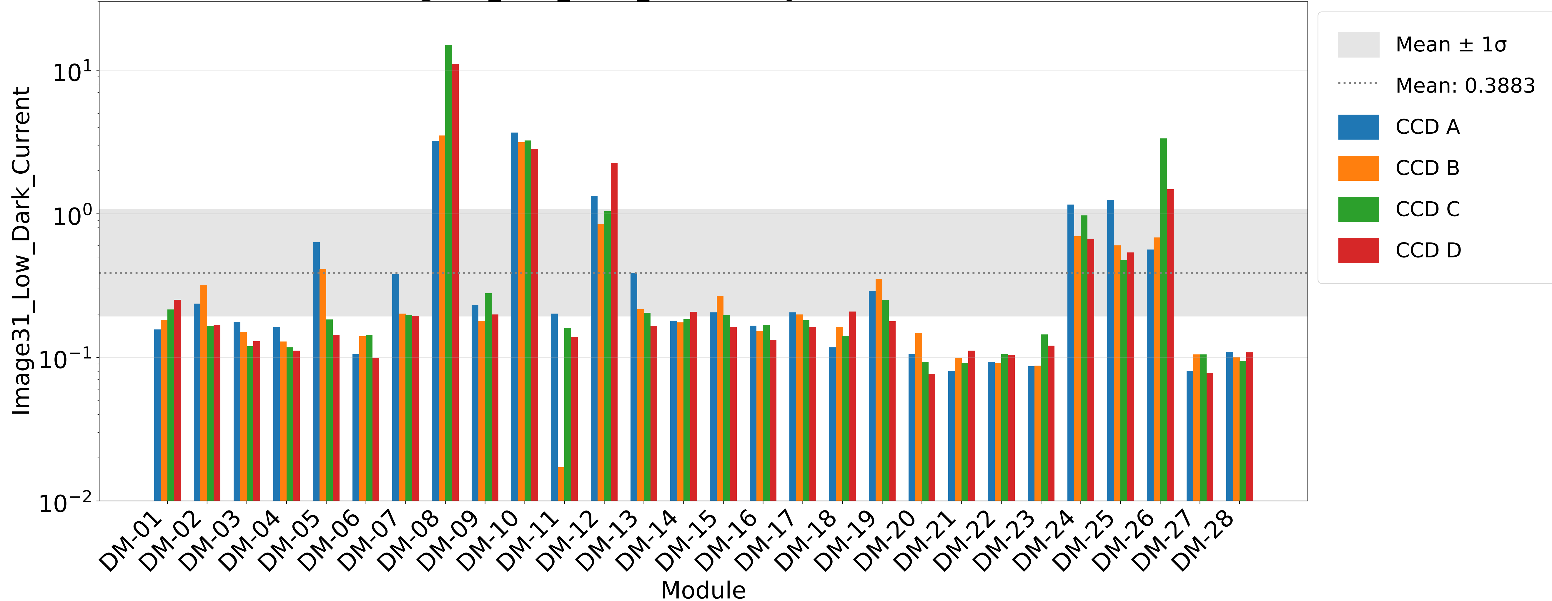
Image31_Low_Dark_Current by Module and CCD
