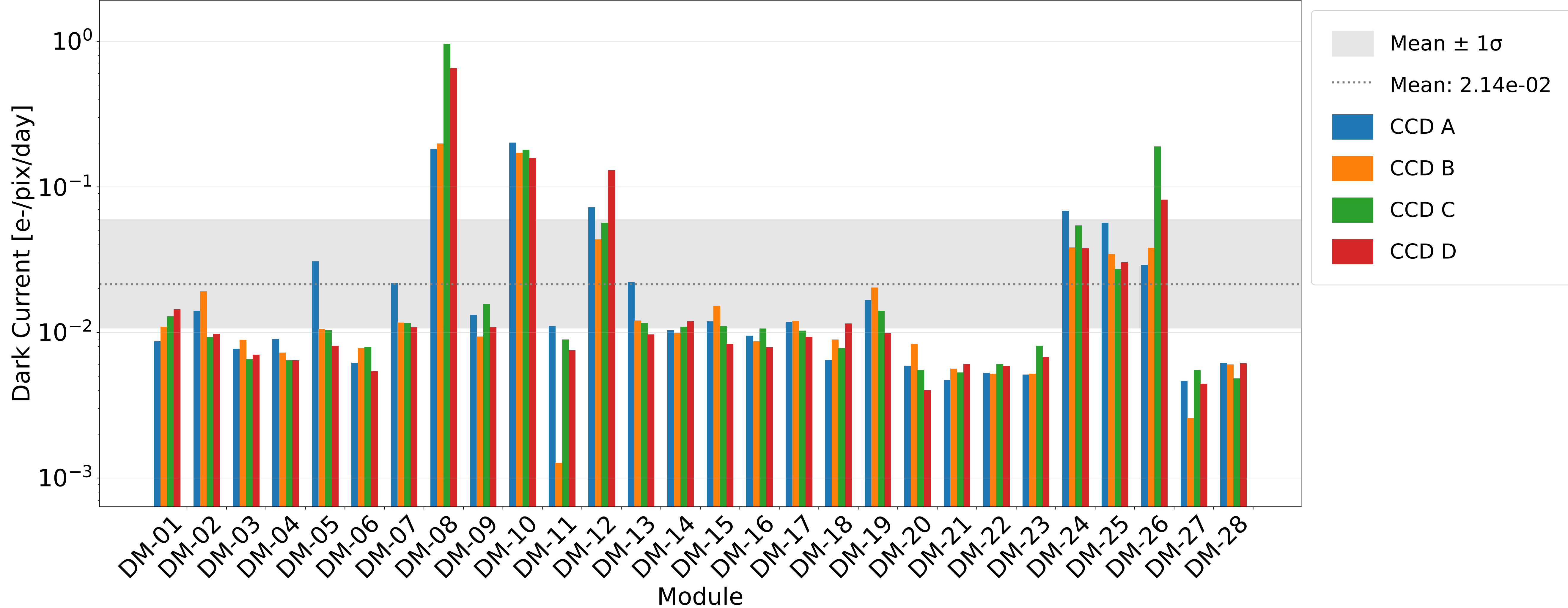
Dark Current from 500-Skip SR Image at 135K
