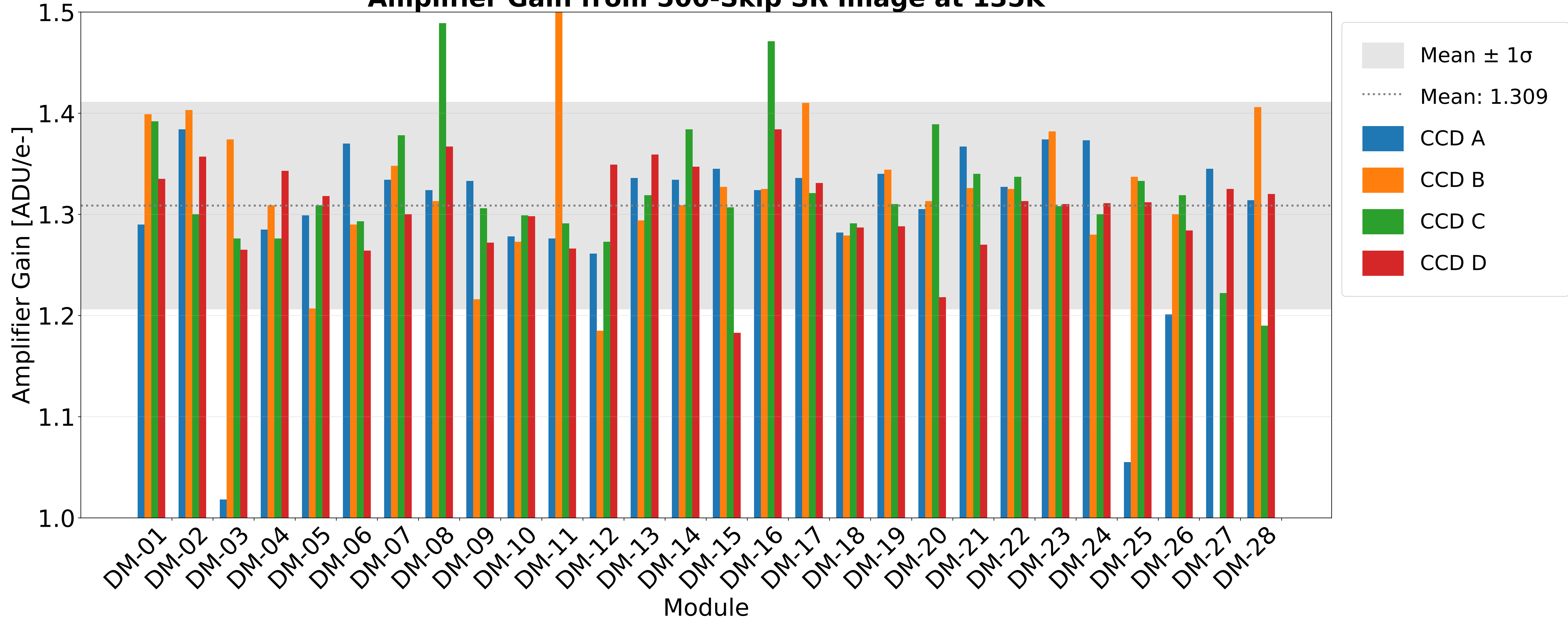
Amplifier Gain from 500-Skip SR Image at 135K
