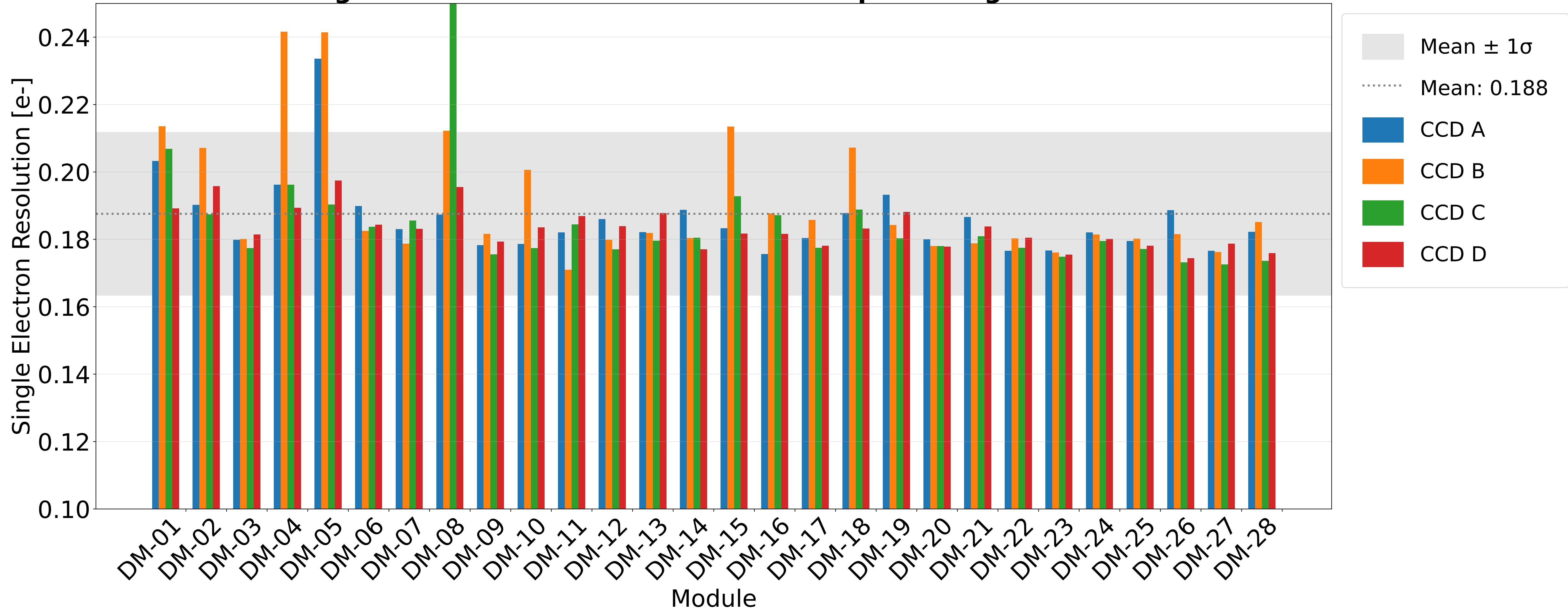
Single Electron Resolution from 500-Skip SR Image at 135K
