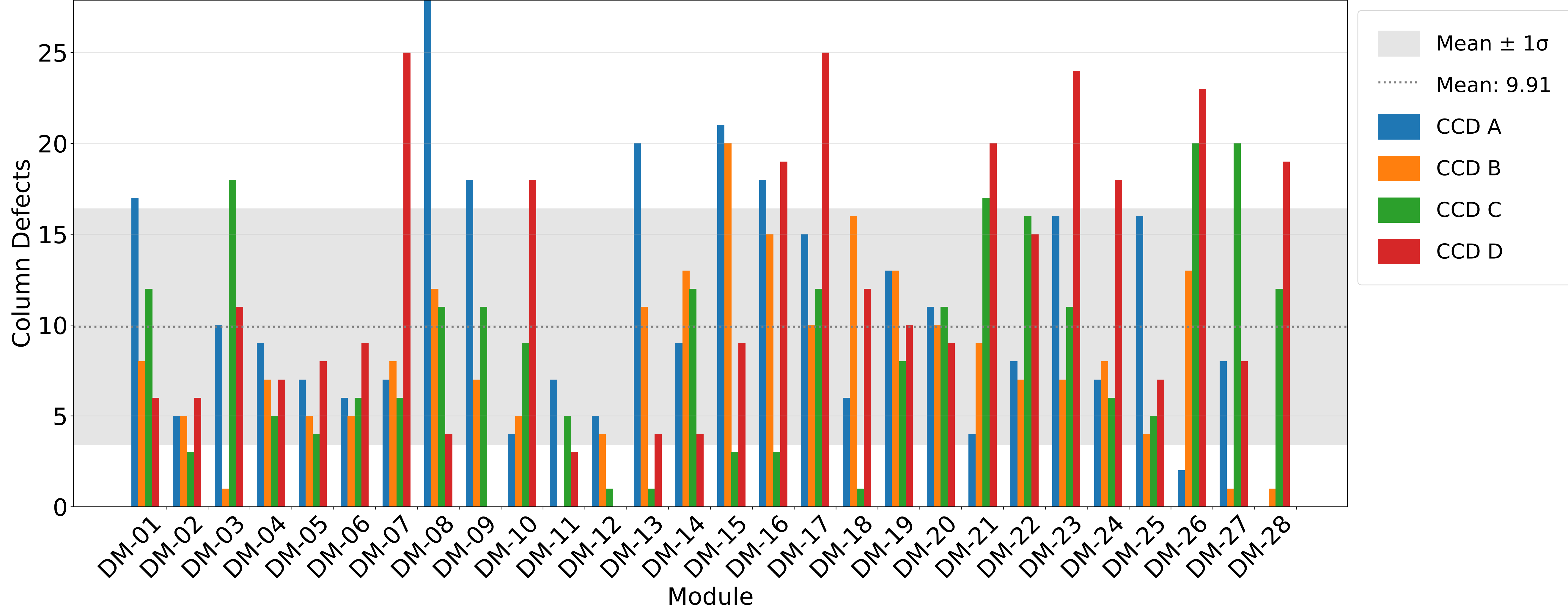
Column Defects from Full Composite Image at 185 K
