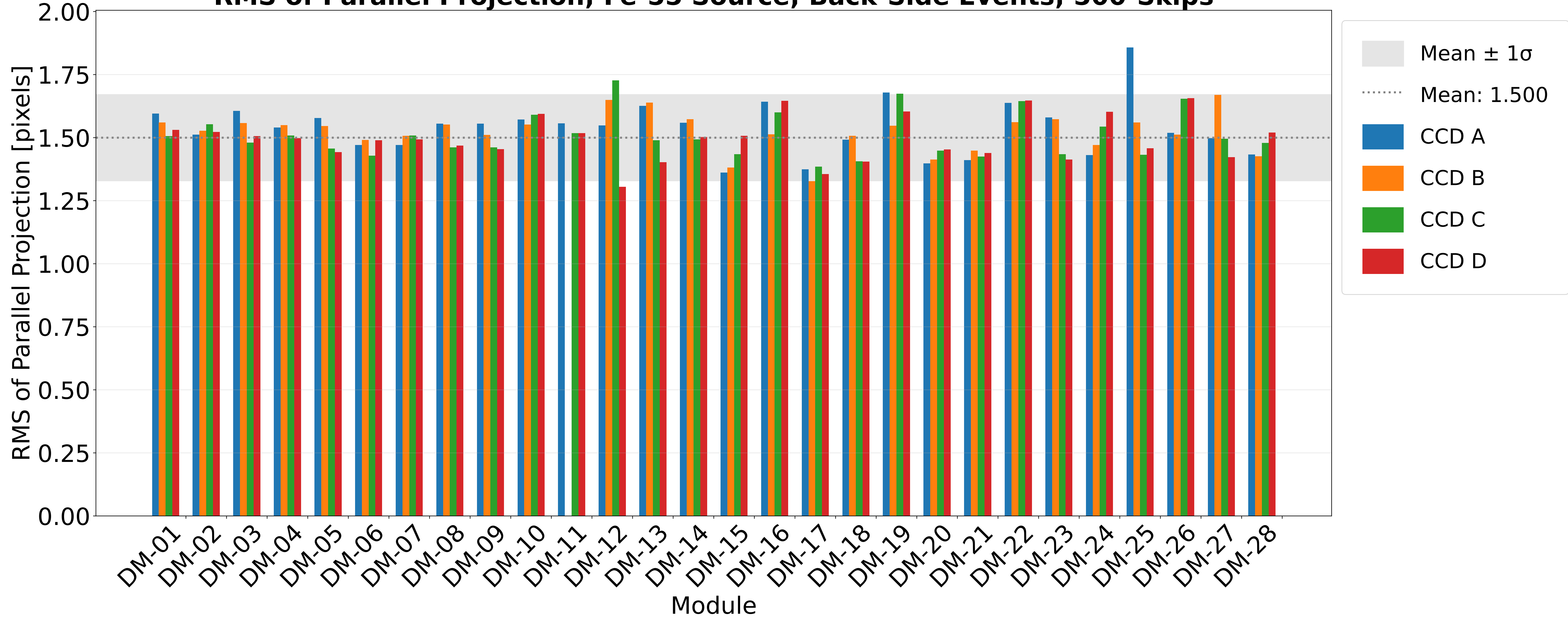
RMS of Parallel Projection; Fe-55 Source; Back-Side Events; 500-Skips
