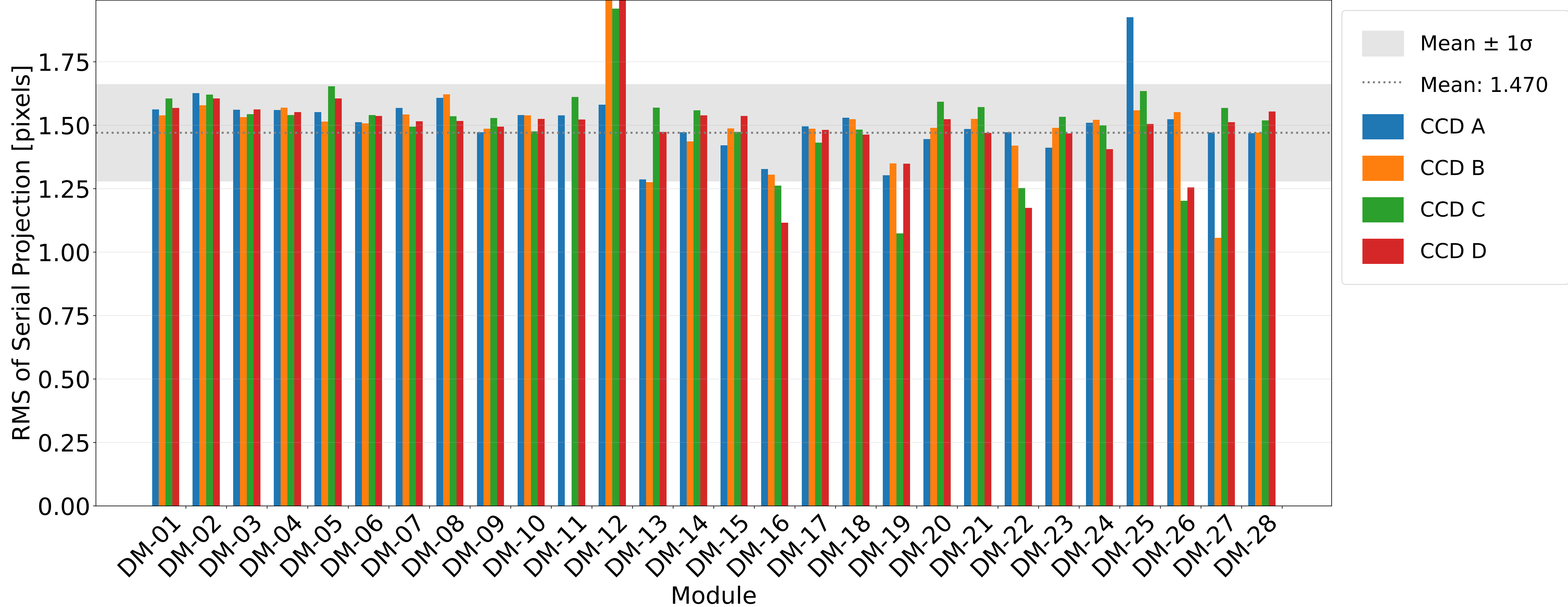
RMS of Serial Projection; Fe-55 Source; Back-Side Events; 500-Skips
