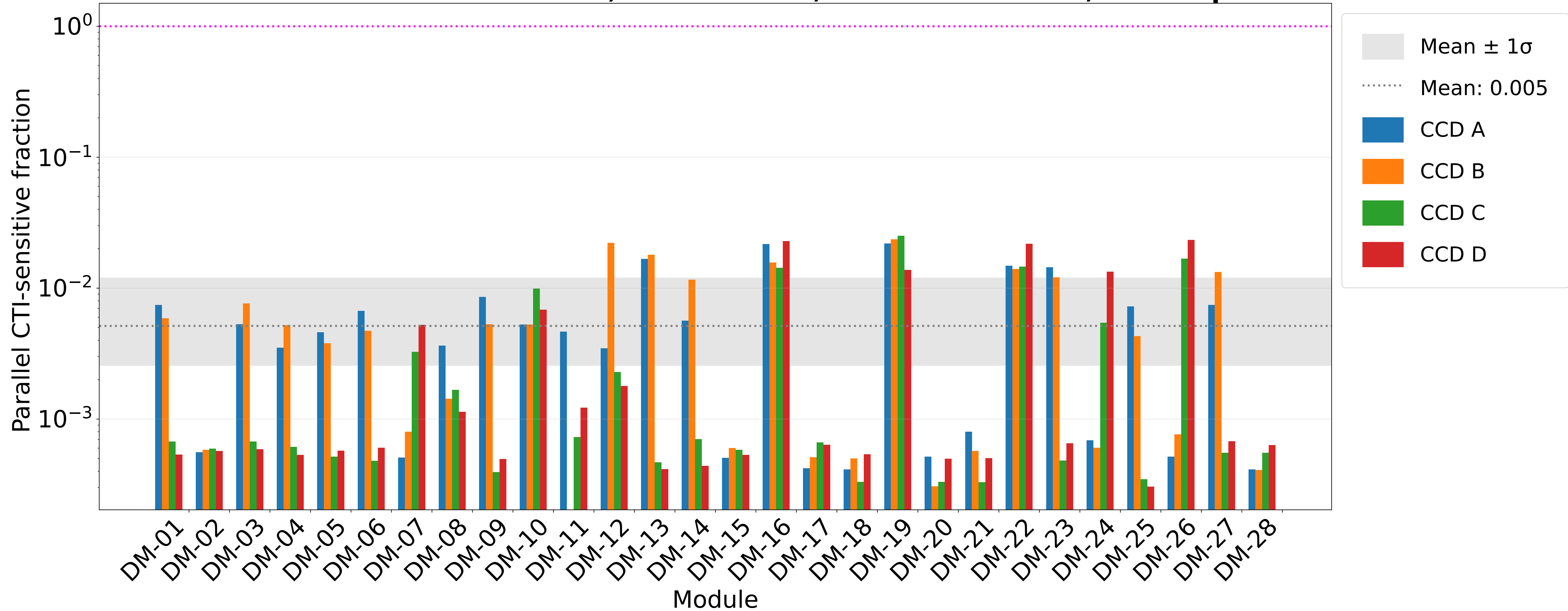
Parallel CTI-sensitive fraction; Fe-55 Source; Front-Side Events; 500-Skips
