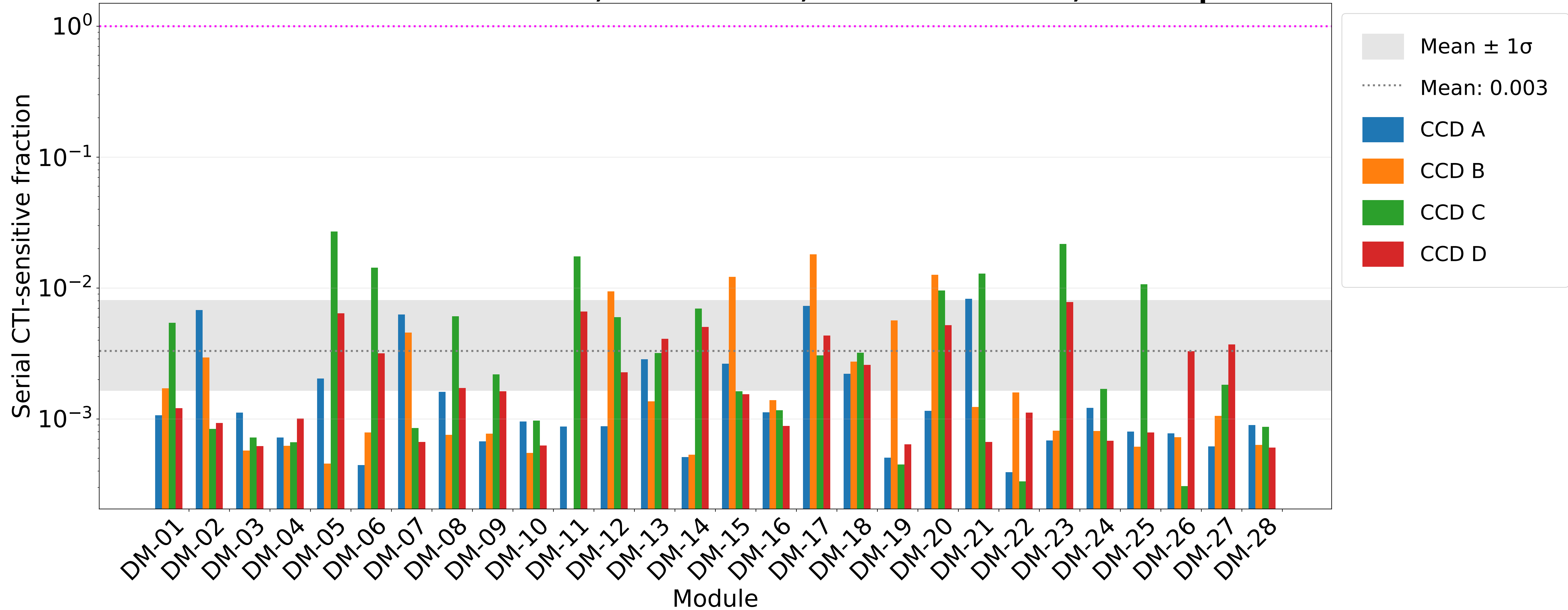
Serial CTI-sensitive fraction; Fe-55 Source; Front-Side Events; 500-Skips
