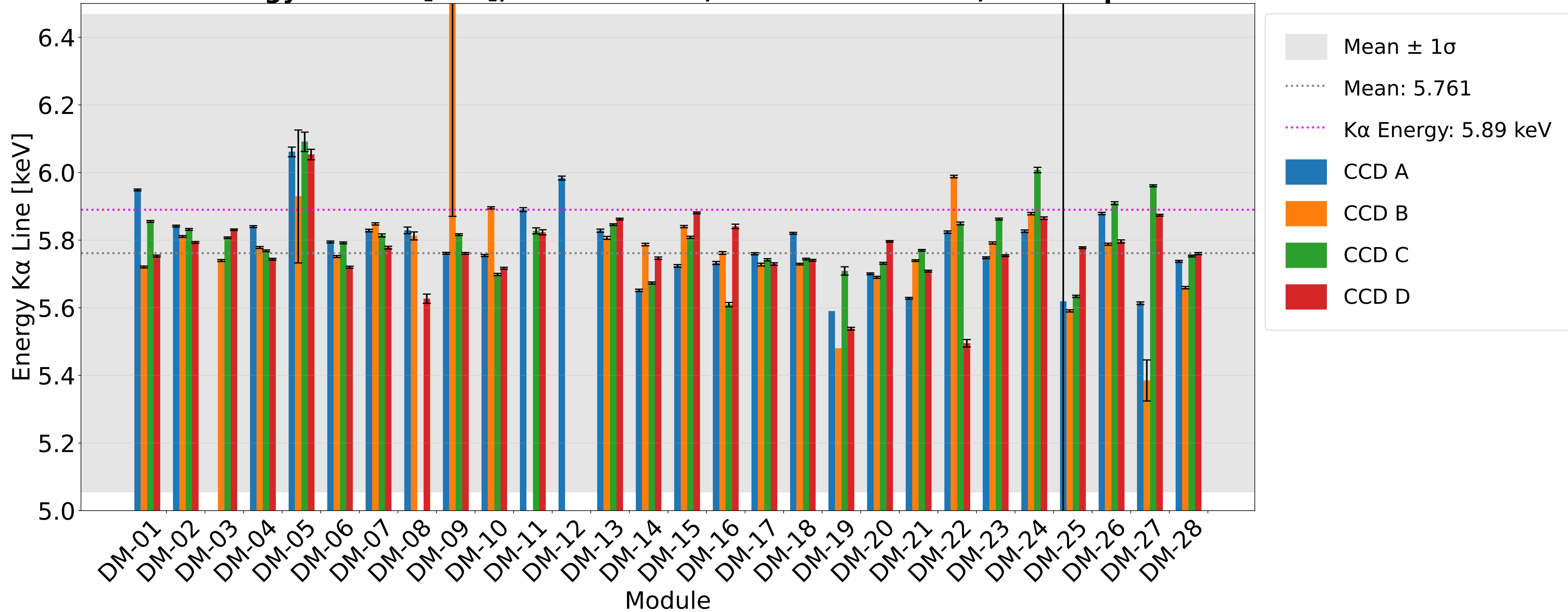
Energy K \alpha Line [keV]; Fe-55 Source; Front-Side Events; 500-Skips
