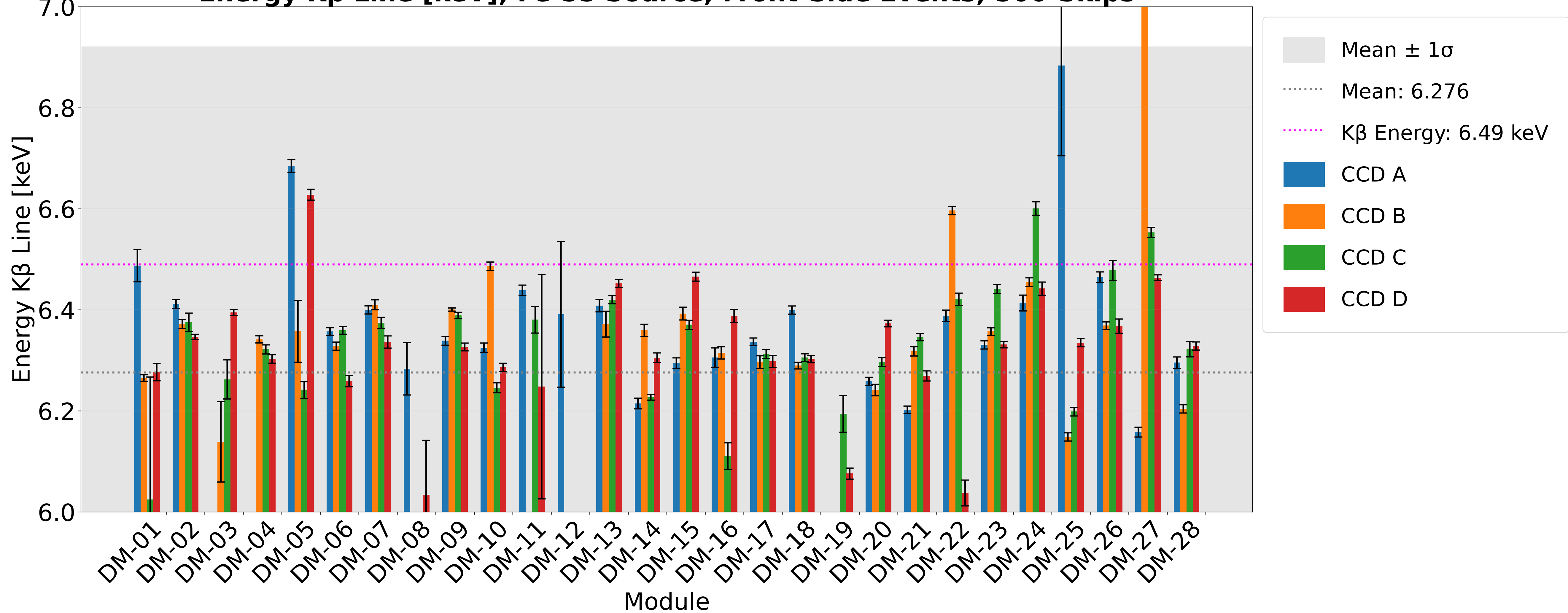
Energy K \beta Line [keV]; Fe-55 Source; Front-Side Events; 500-Skips
