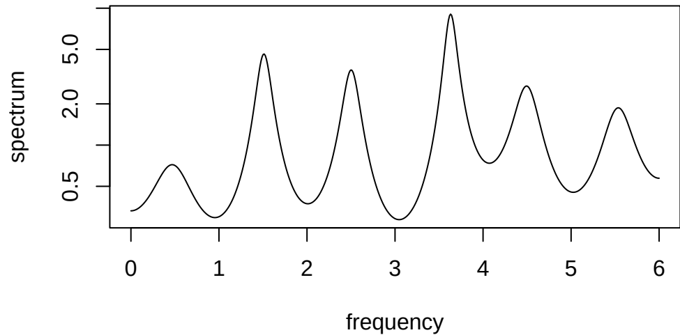
Series: x AR (12) spectrum
