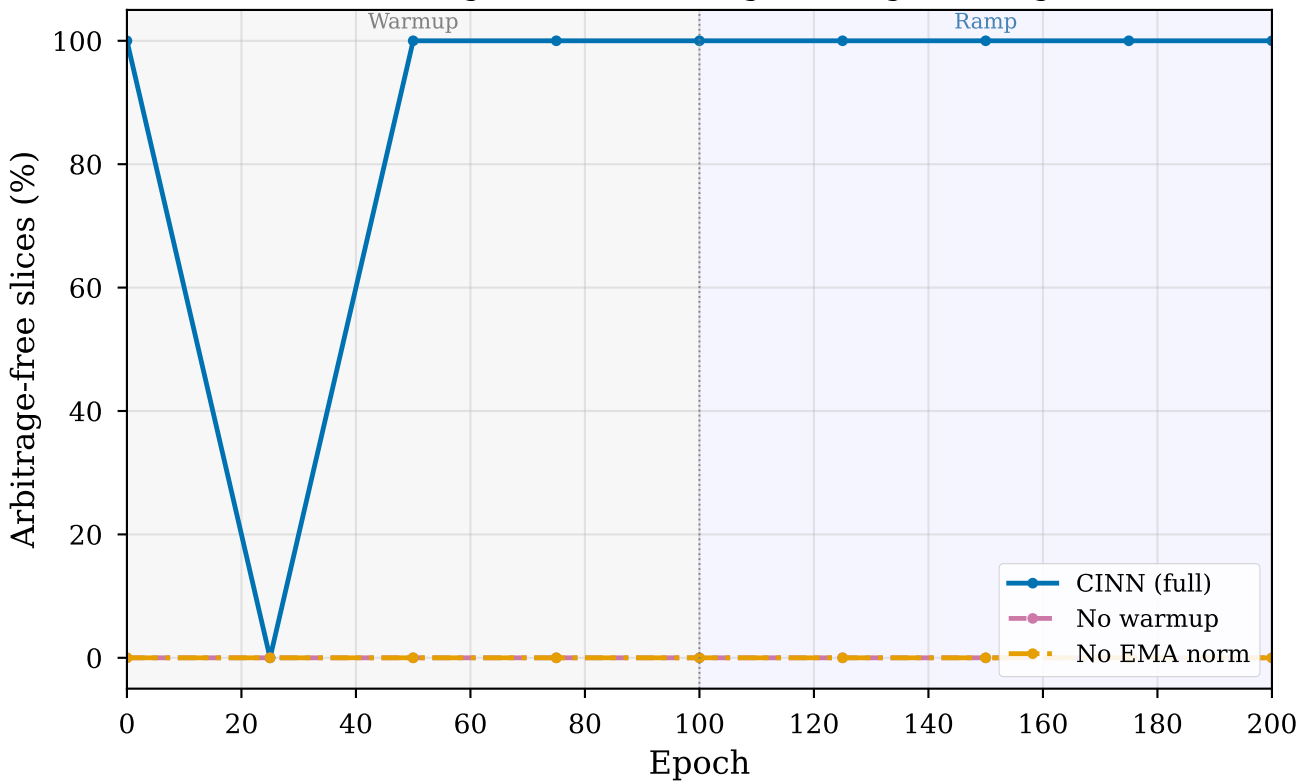
Arbitrage-Free Percentage During Training
