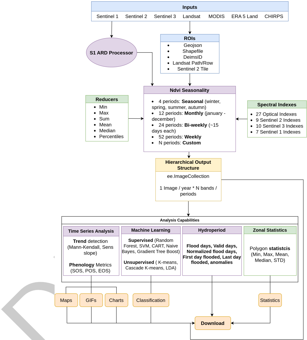
Figure 1: Ndvi2Gif workflow architecture and capabilities. Color coding: Blue — input data sources and ROI specification; Green — processing operations; Purple — main analysis classes; Orange — download-ready output products.
