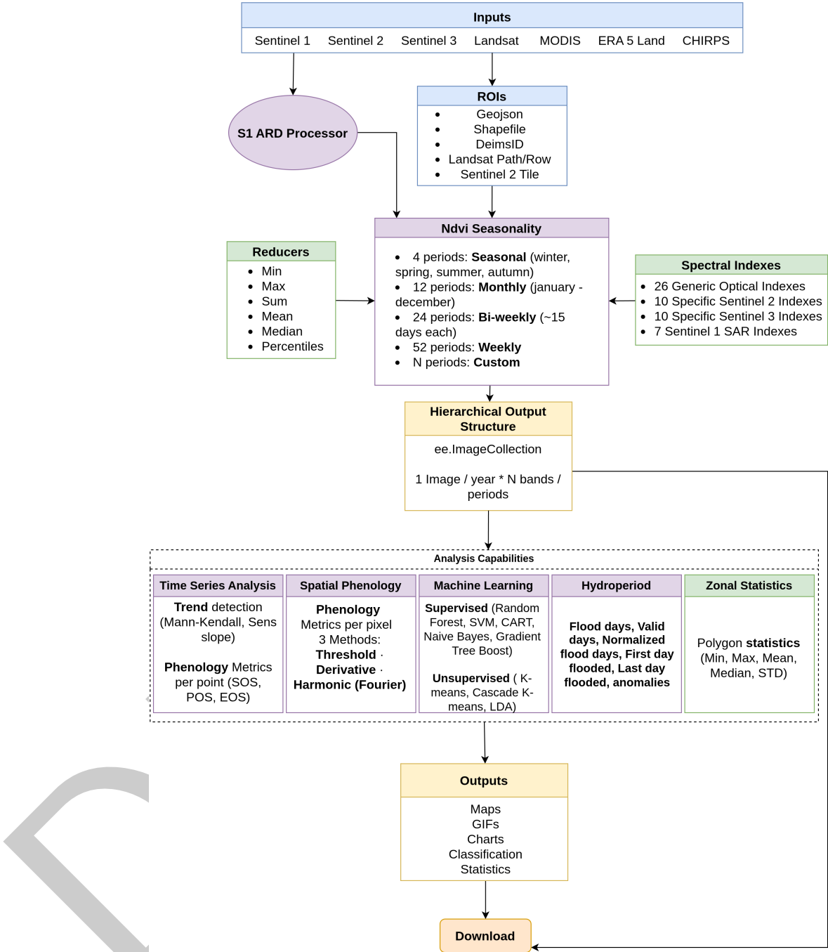
Figure 1: Ndvigif workflow architecture and capabilities. Color coding: Blue — input data sources and ROI specification; Green — processing operations; Purple — main analysis classes; Orange — download-ready output products.
