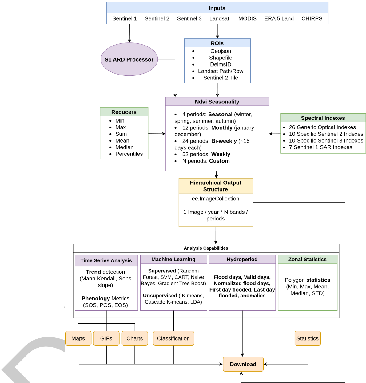
Figure 1: Ndvi2Gif workflow architecture and capabilities. Color coding: Blue — input data sources and ROI specification; Green — processing operations; Purple — main analysis classes; Orange — download-ready output products.
