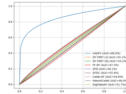
(e) HeadPose
