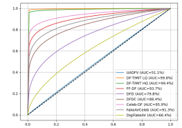
(f) F3-Net
