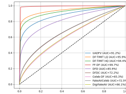
(c) Xception-c23
