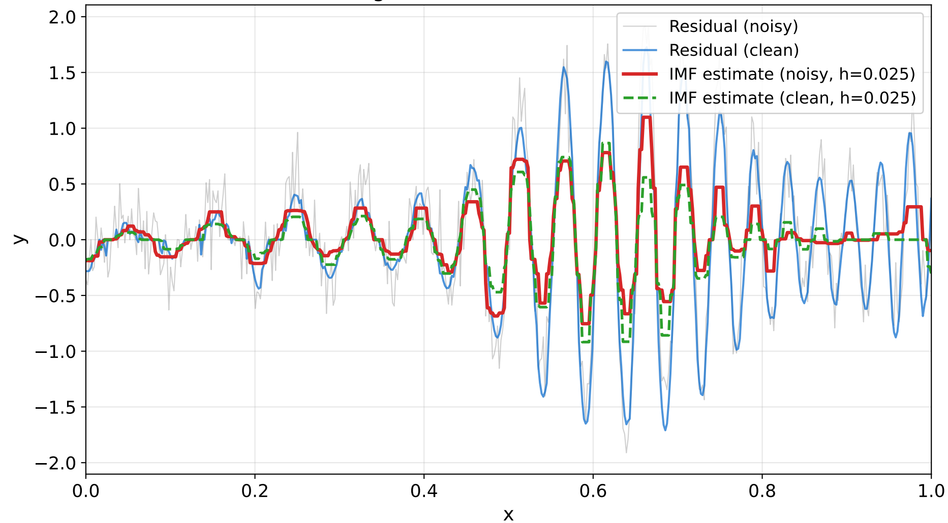
Sifting Iteration 5: h = 0.025 ( h_1/4 )
