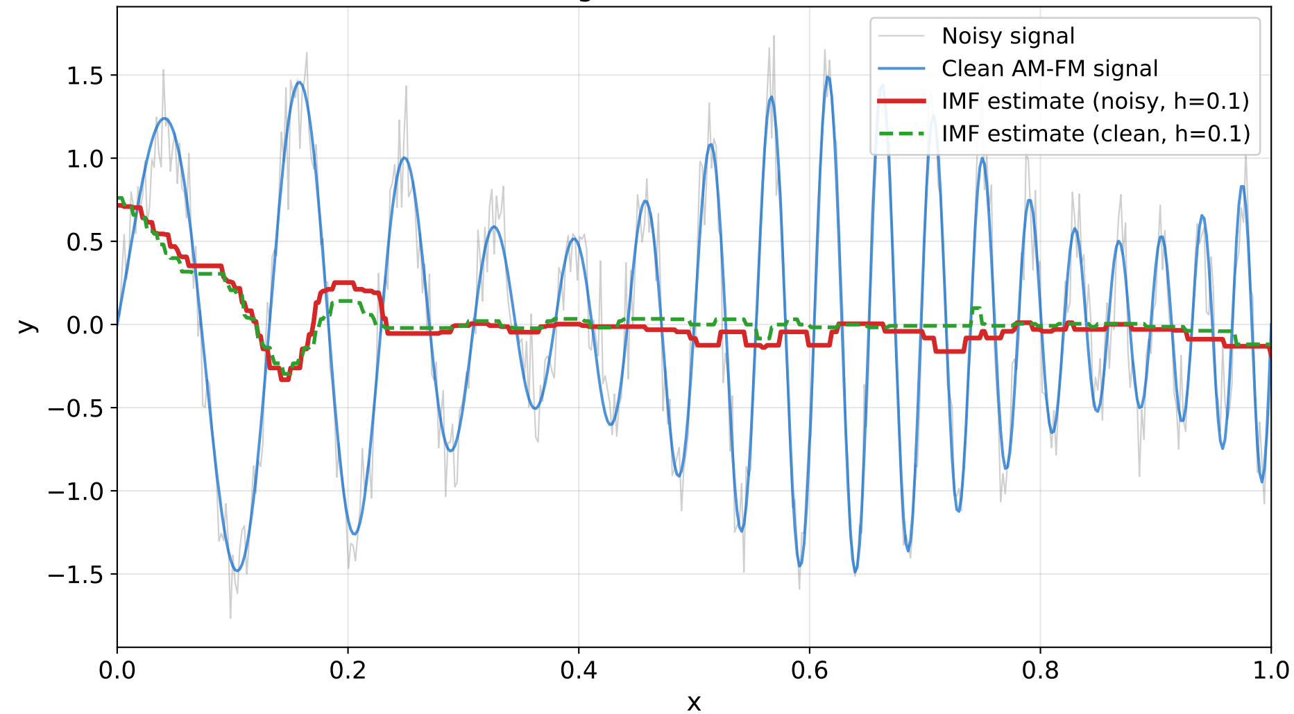
Sifting Iteration 1: h = 0.1
