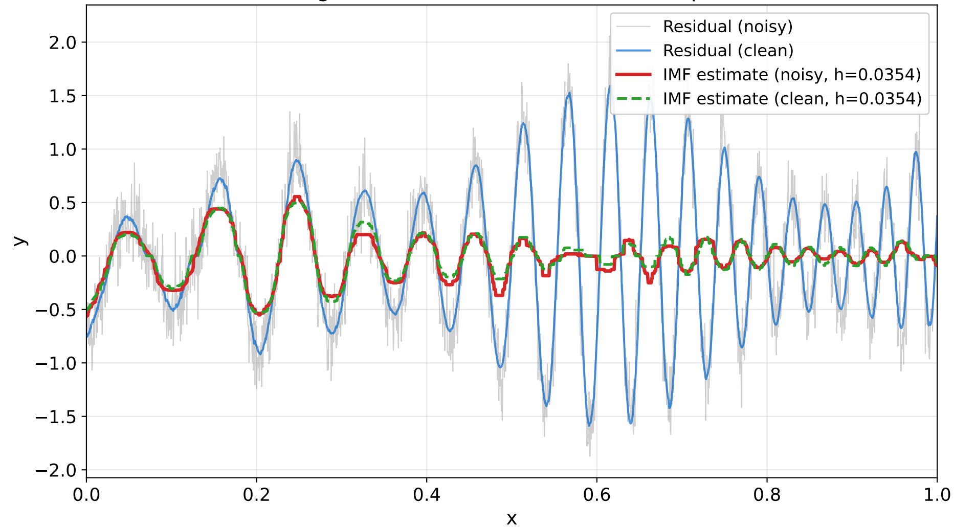
Sifting Iteration 4: h = 0.0354 ( h/(2*\sqrt{2}) )
