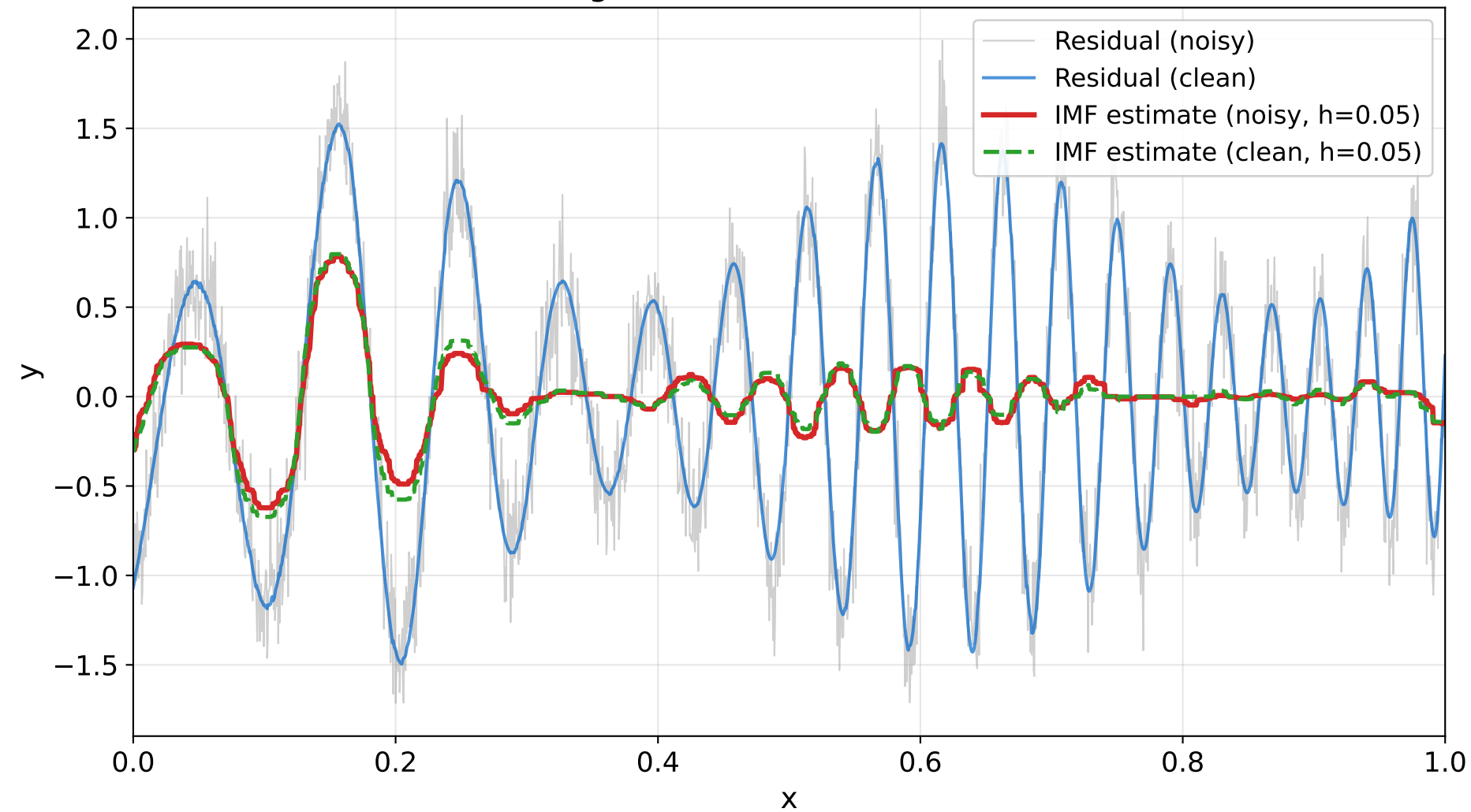
Sifting Iteration 3: h = 0.05 ( h1/2 )
