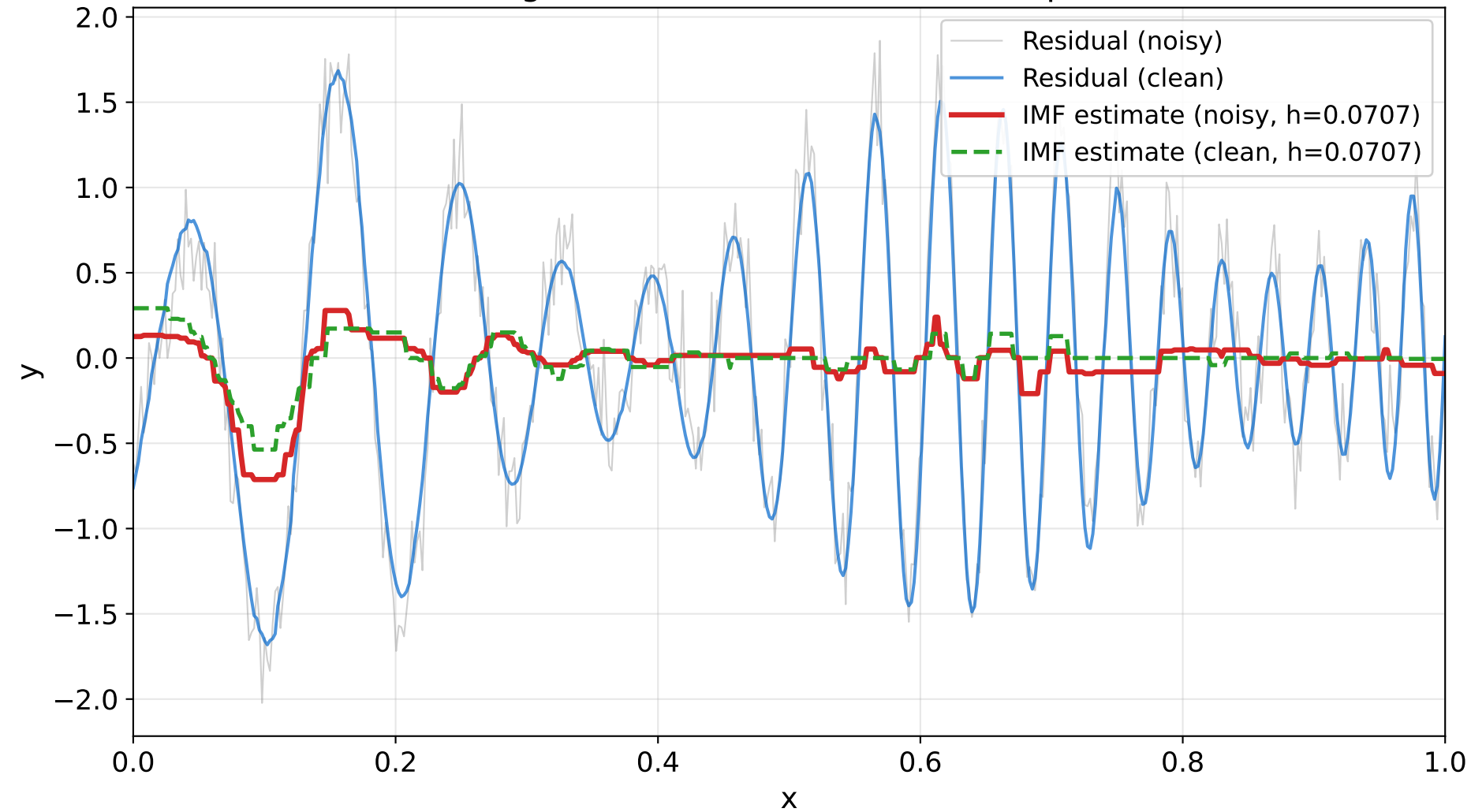
Sifting Iteration 2: h = 0.0707 ( h_1/\sqrt{2} )
