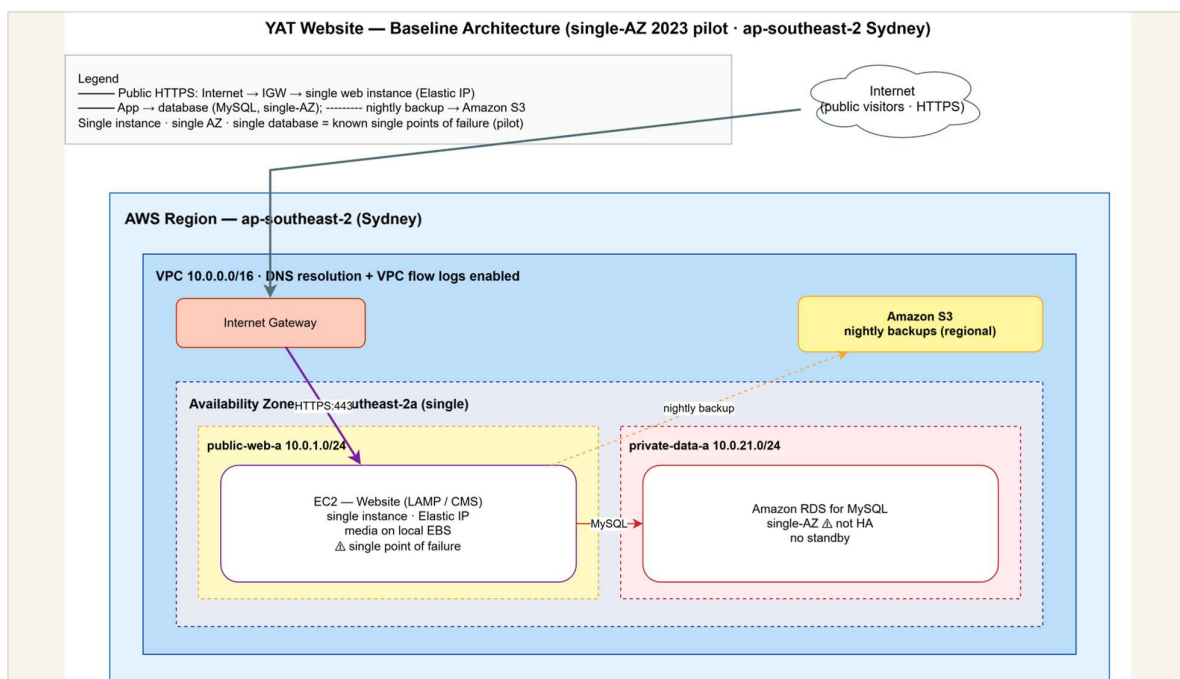
Figure 4.4 — Website baseline network topology (single-AZ, single instance).
