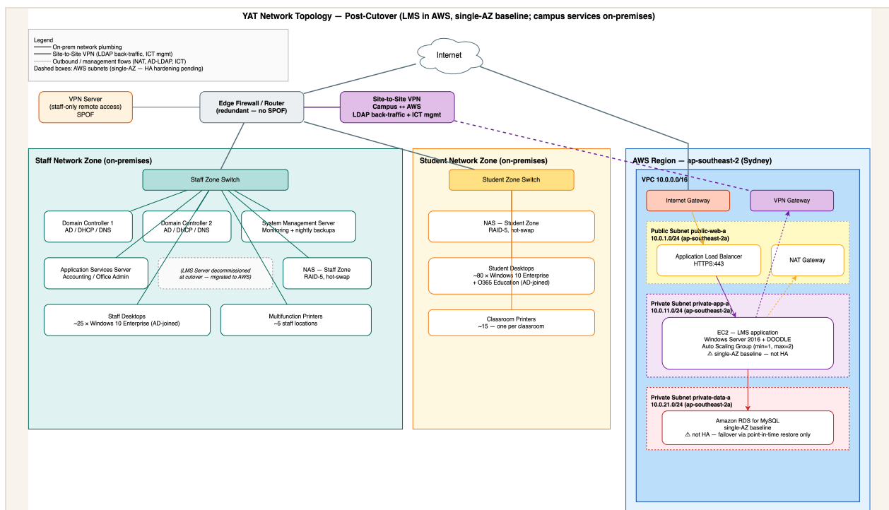
Figure 4.4 — LMS baseline network topology (single-AZ).
