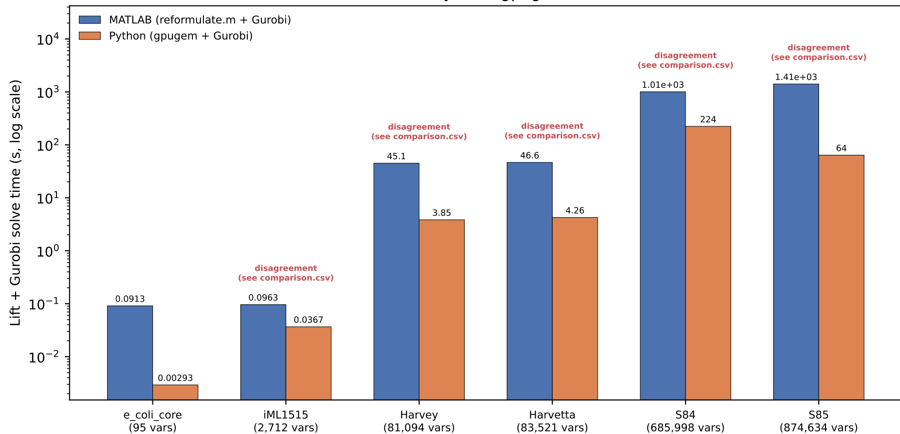
MATLAB (reformulate.m) vs Python (gpugem) lifted-model solve time
