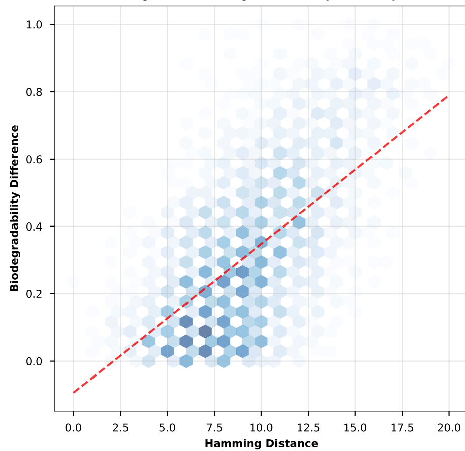
S4MOGAligned: Hamming Distance\n \rho=0.571 , p<0.001
