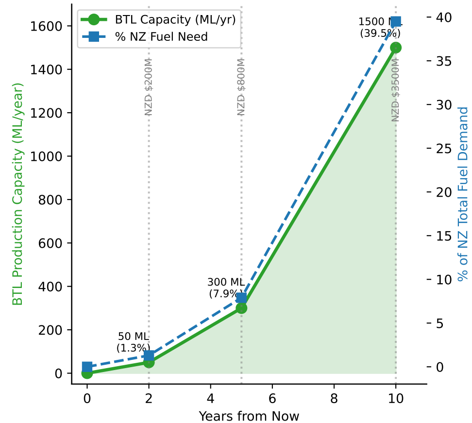
(b) NZ BTL Development Roadmap Scion/Forestry Biomass to Liquid Fuels
