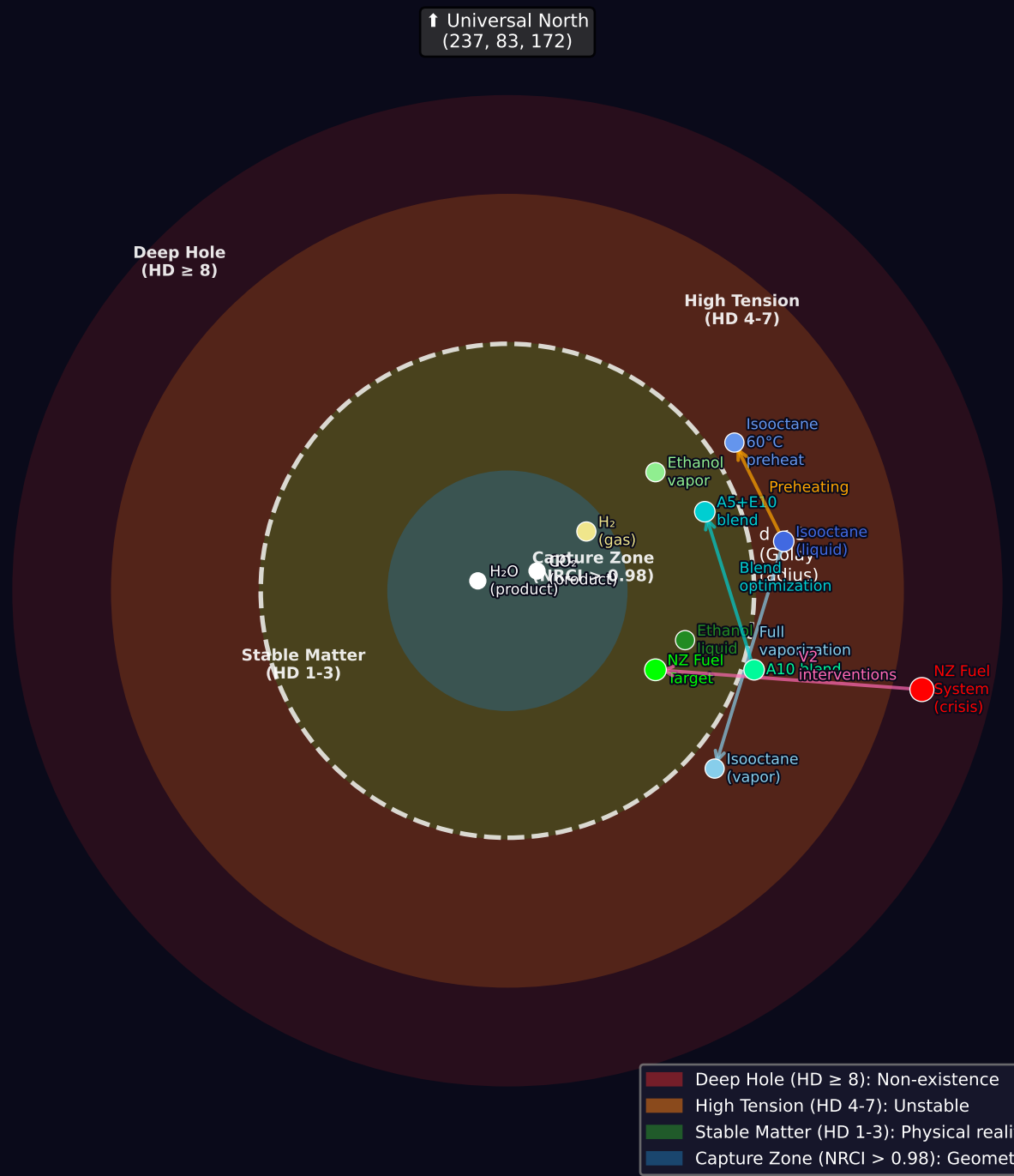
Figure 5: UBP Leech Lattice Phase Map — NZ Fuel Combustion Manifold Molecular States as Codewords in \Lambda_{24}
