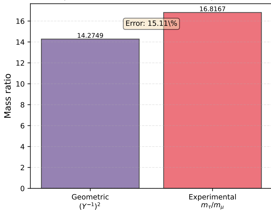
(c) \tau/\mu Mass Ratio: Geometric vs Experimental
