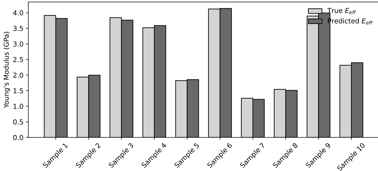
True vs. Predicted Effective Stiffness (10 Random Samples)
