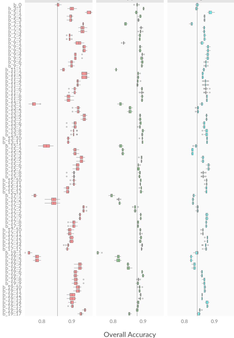
Order::Window size
