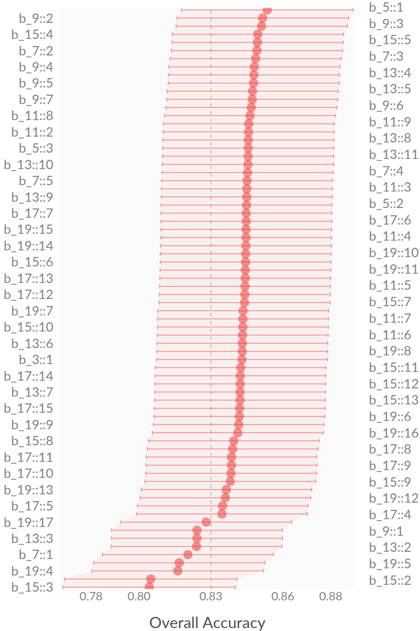
Order::Window size
