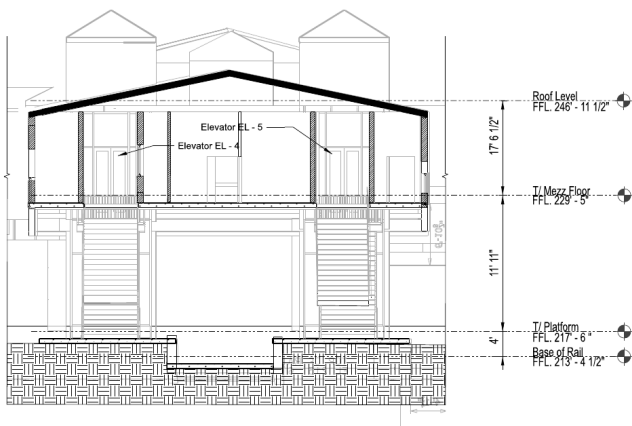
2 J/Z STATION - TRASVERSE SECTION 1/8" = 1'-0"
