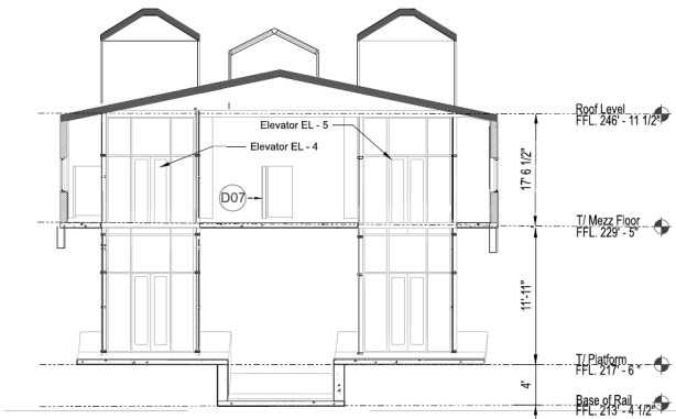
1 J/Z STATION - TRASVERSE SECTION 1/8" = 1'-0"
