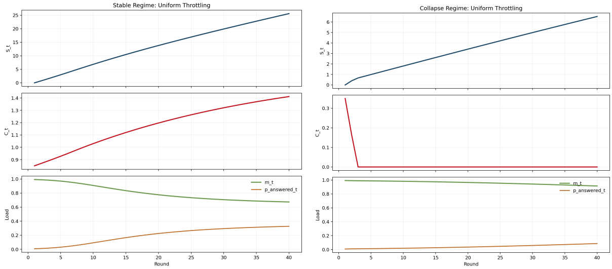
Figure 7: Time-series examples. Left: stable regime, where capacity remains healthy and knowledge grows steadily. Right: collapse regime, where overload damages capacity and the system falls into a bad state.
