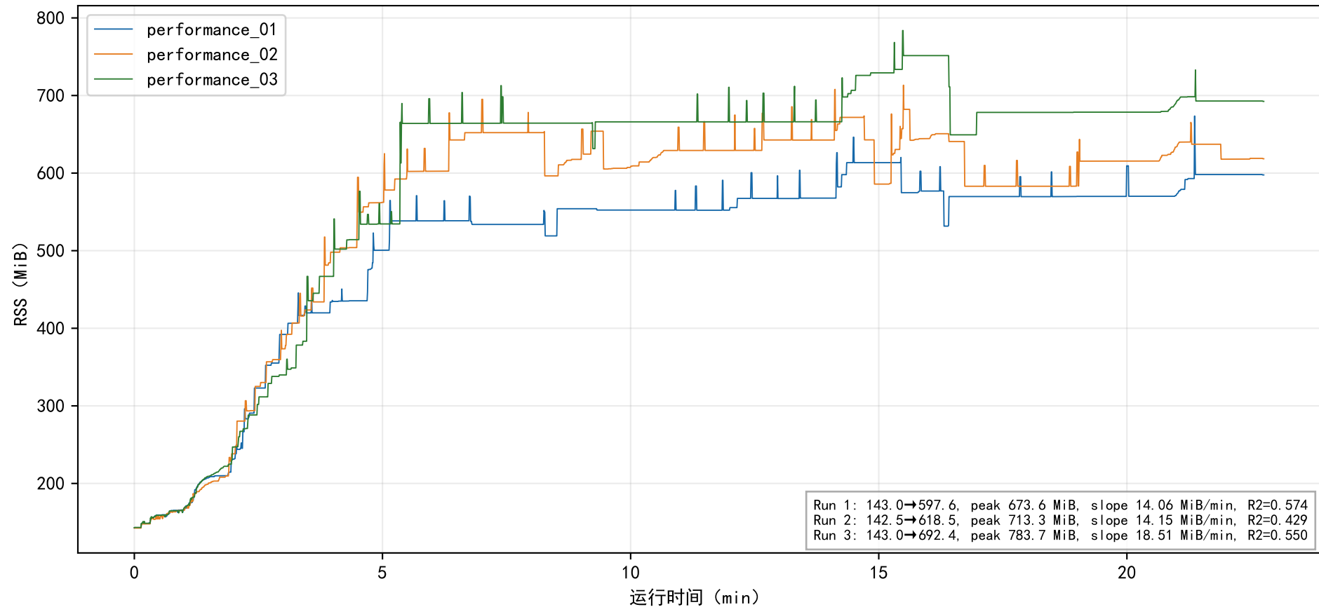
AMtown01 FAST-LI02 进程 RSS 随时间变化 (原始样本)
