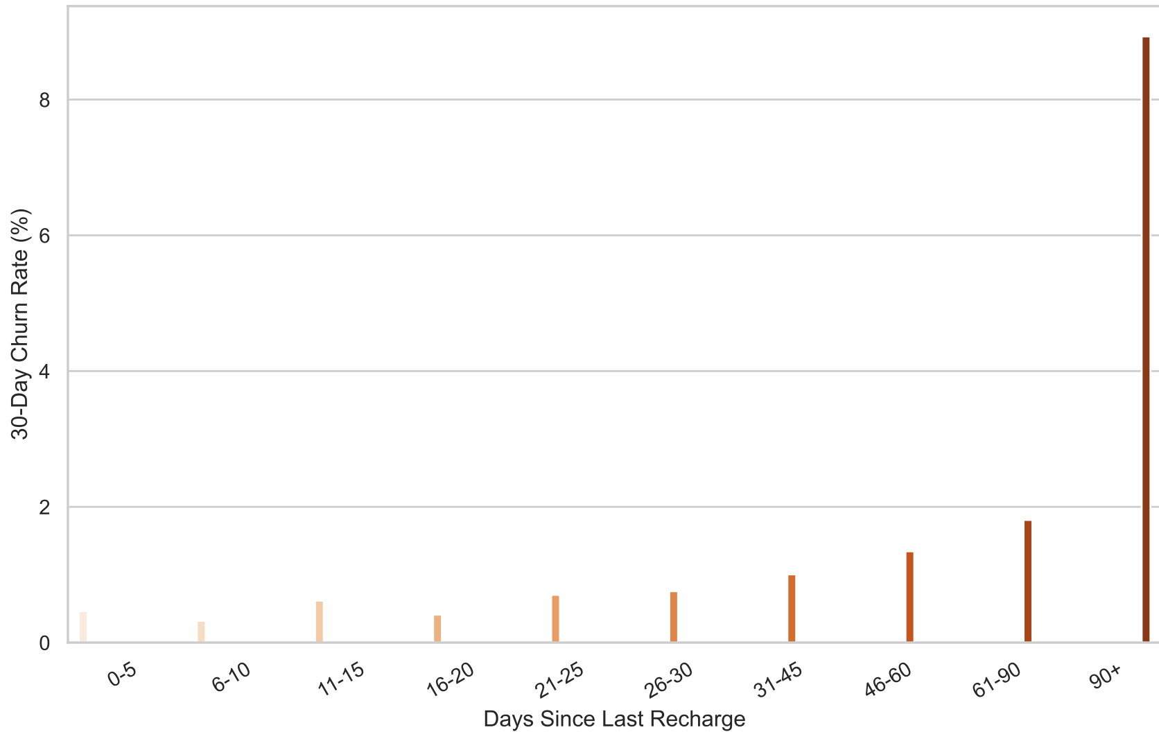
Churn Rate vs. Recharge Gap (Silent Churn Threshold)
