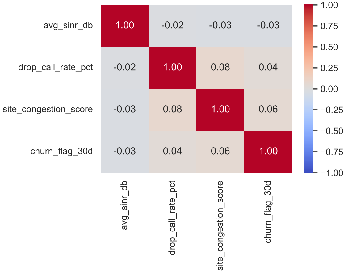
Network KPI vs. Churn Correlation Matrix
