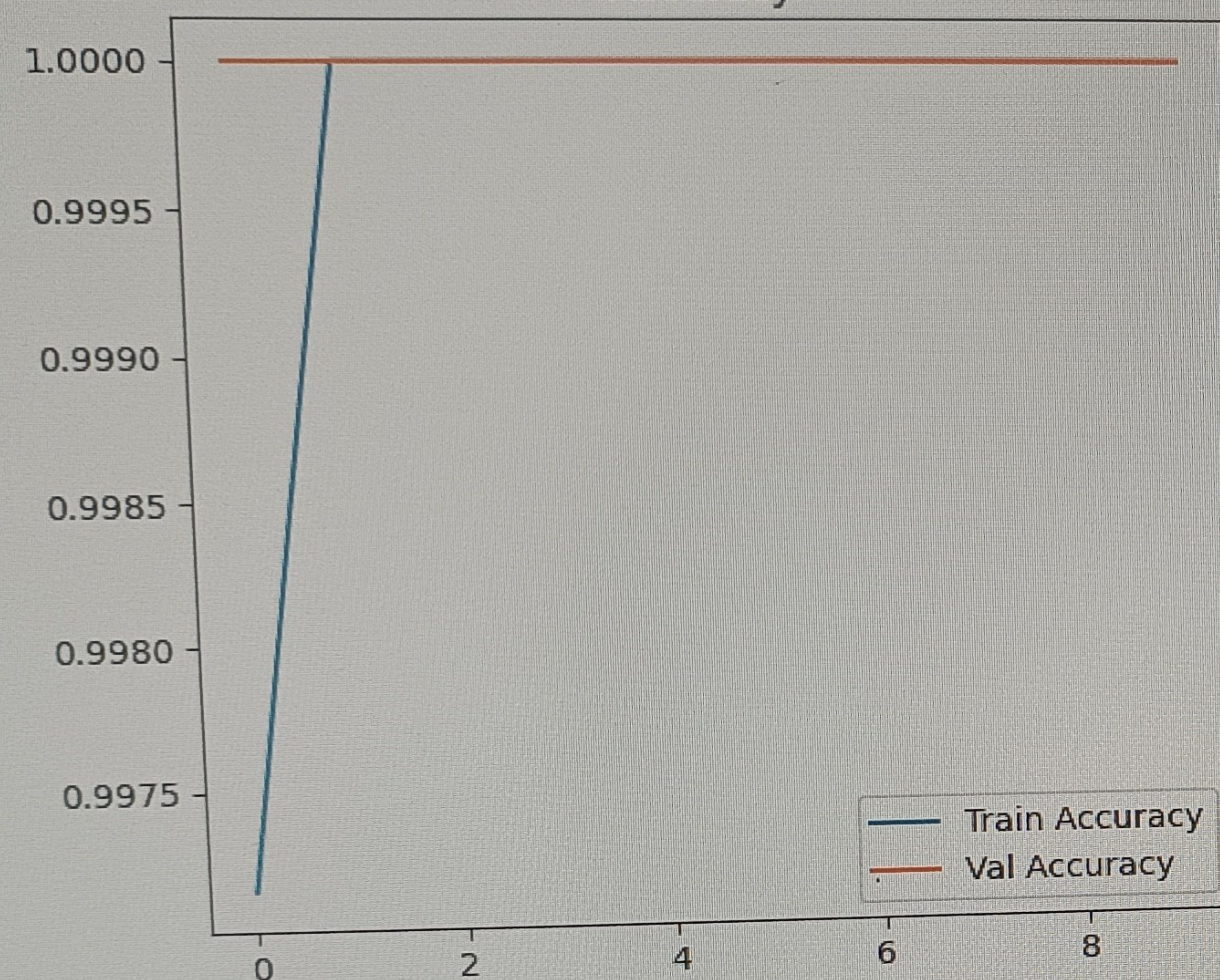
Accuracy
