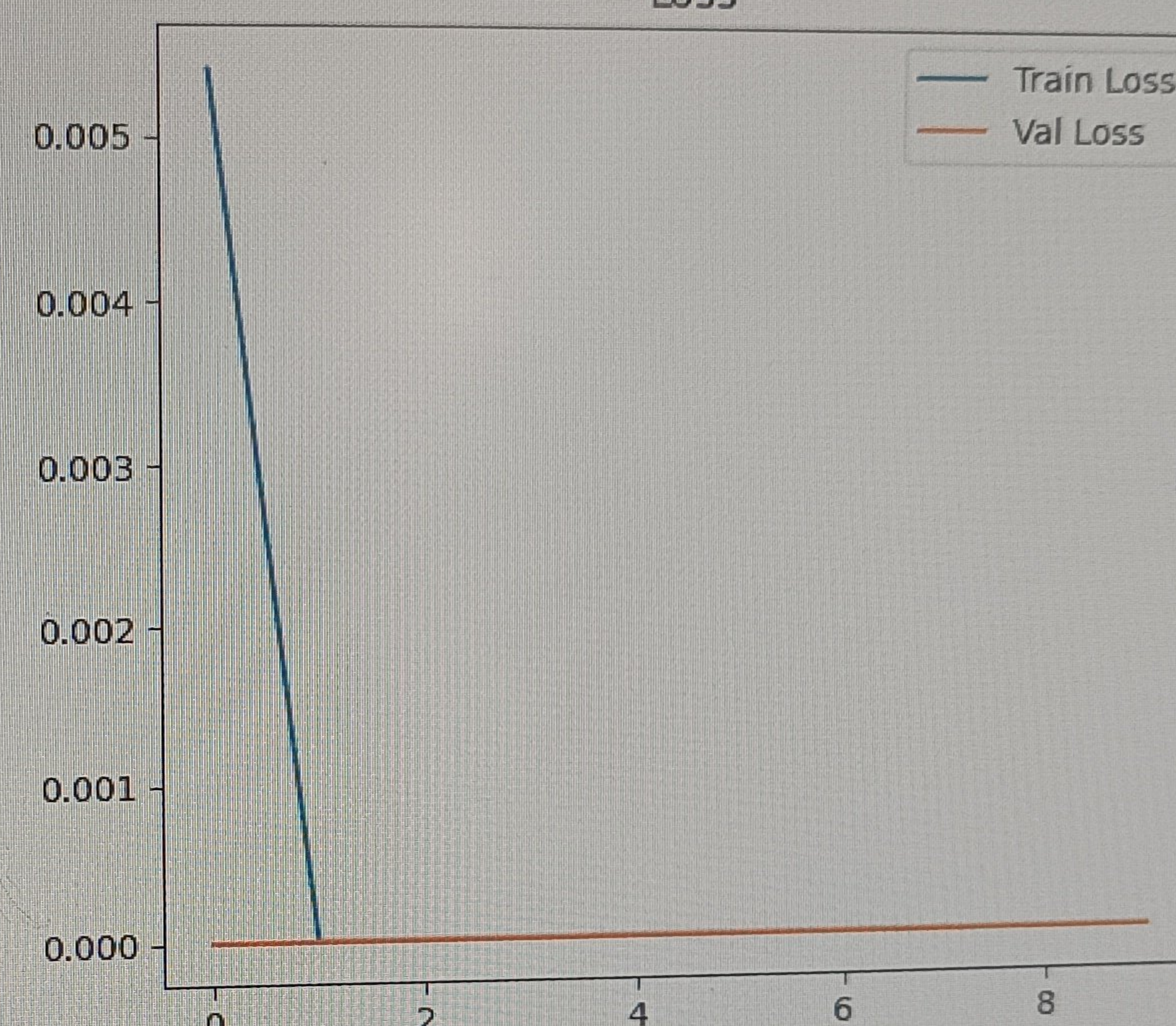
Loss
