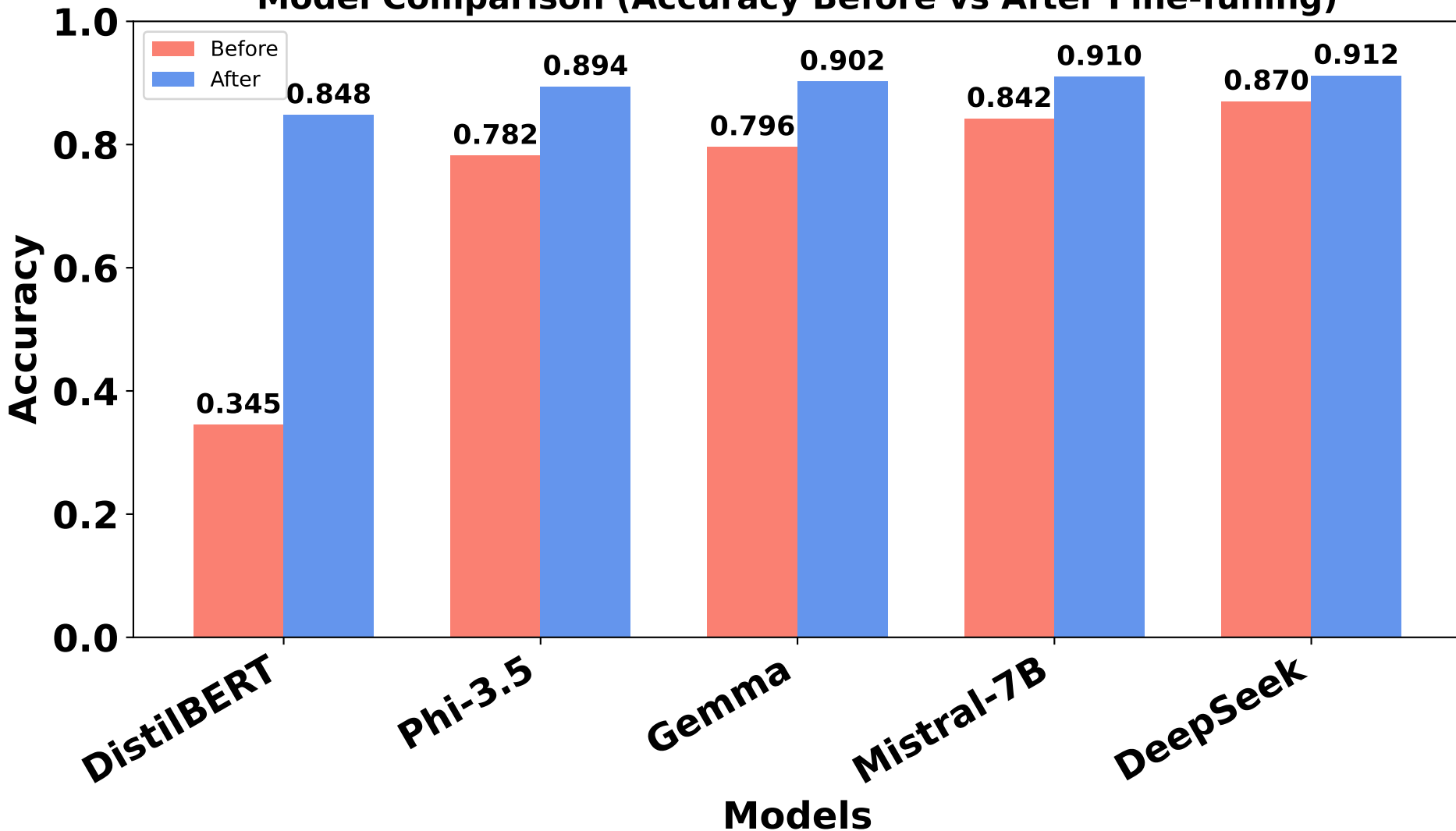
Model Comparison (Accuracy Before vs After Fine-Tuning)
