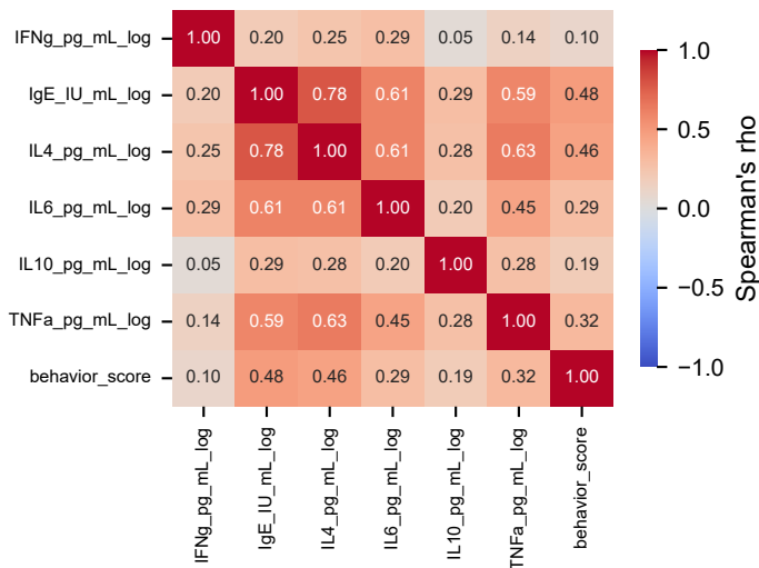
Correlation structure
