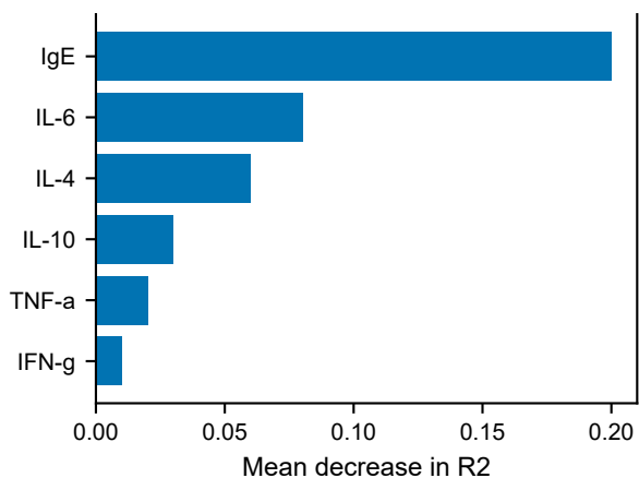
Permutation importance
