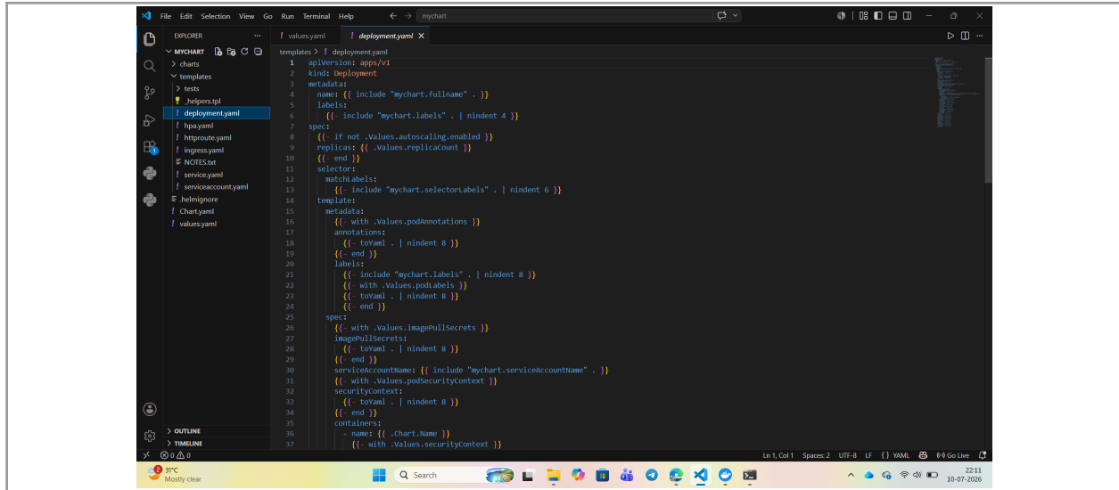
Figure 14: Custom Helm chart deployment.yaml template using Helm templating functions
