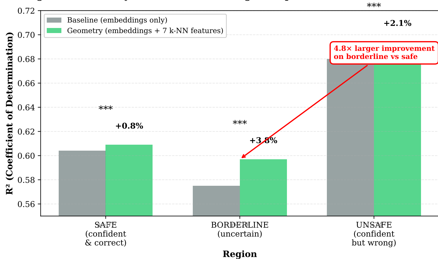
Figure 1: Geometry Features Provide Largest Improvement on Borderline Cases
