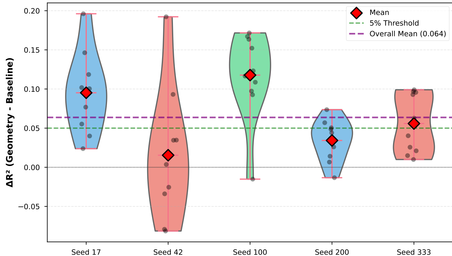
Per-Seed Performance Distribution (10 runs each)
