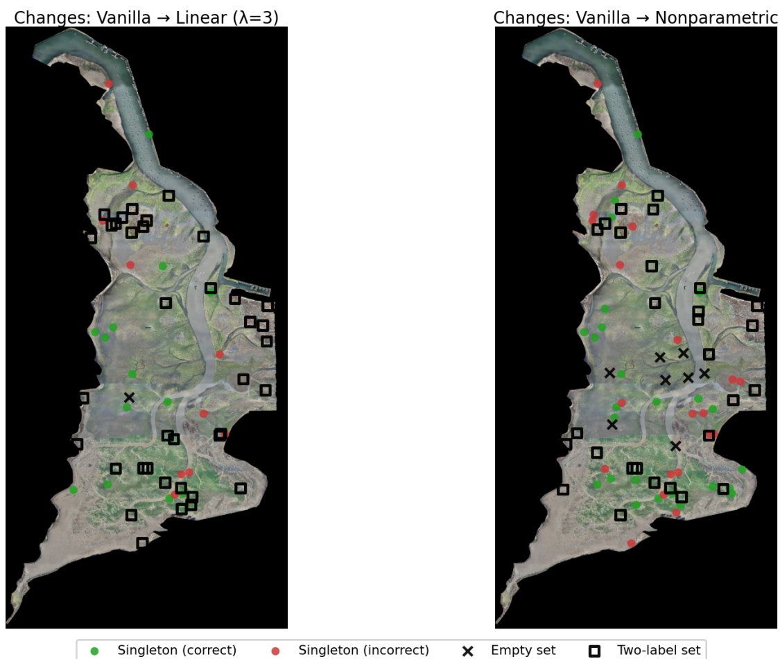
Figure 4.11: Set composition changes from vanilla for linear ( \lambda = 3 ) and nonparametric methods
