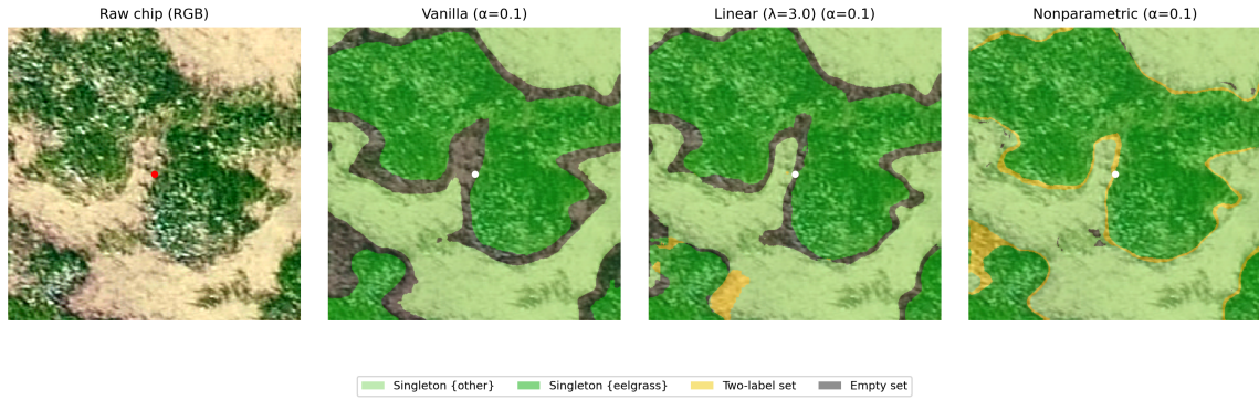
Figure 4.12: Chip-level set prediction comparison on a representative 2022 point (GT = eelgrass). Both vanilla and linear methods return empty sets at that pixel, while the nonparametric method returns the correct singleton {eelgrass}.
