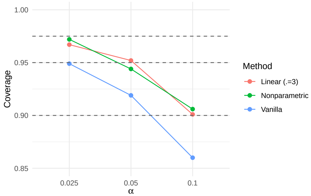
Figure 4.13: Overall coverage on 2022 OOD points across \alpha \in \{0.1, 0.05, 0.025\} for each method. Dashed line shows the target coverage 1 - \alpha .
