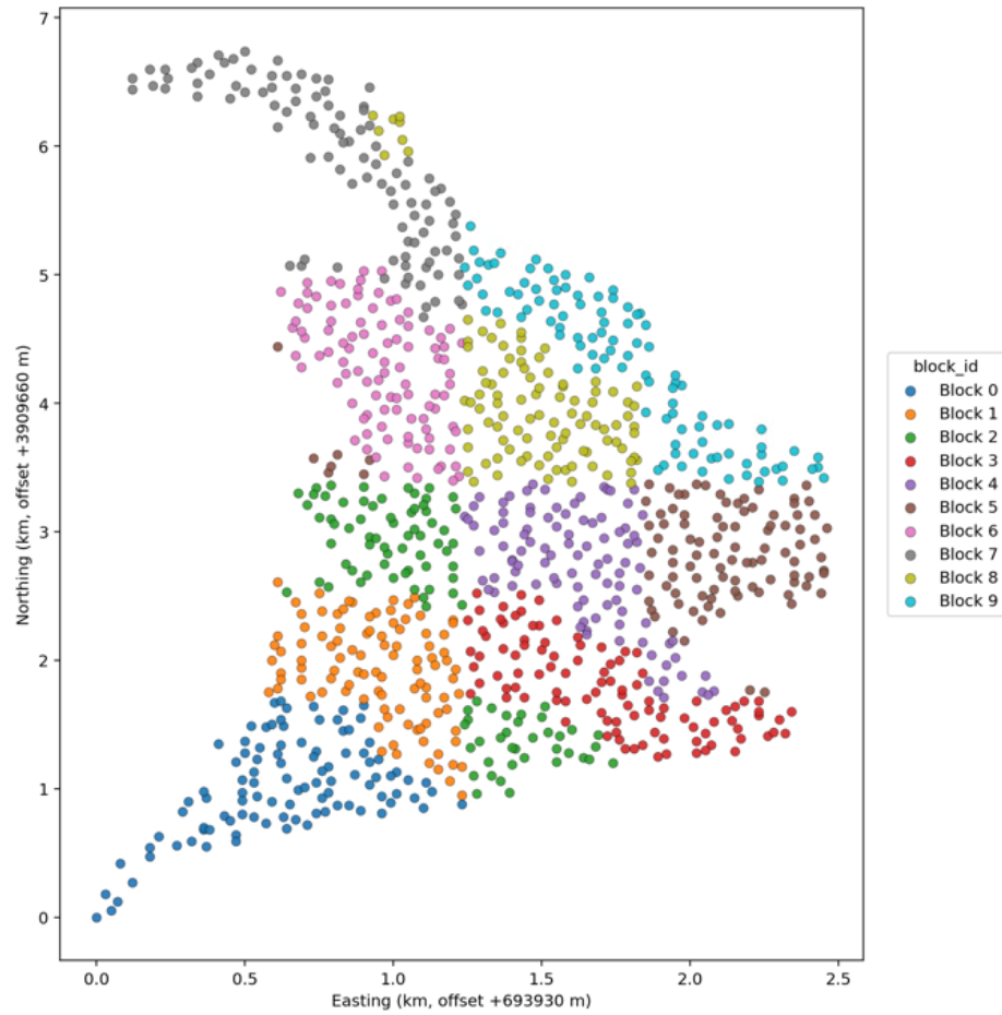
Figure 3.4: Spatial blocks (10 equal-count spatial blocks formed by Morton ordering)
