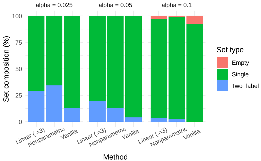
Figure 4.14: Set composition (empty, single, two-label) for each method on 2022 OOD points across \alpha \in \{0.1, 0.05, 0.025\} .
