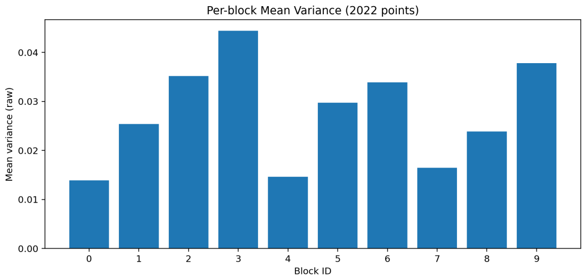
Figure 4.6: Per-block mean variance for 2022 points
