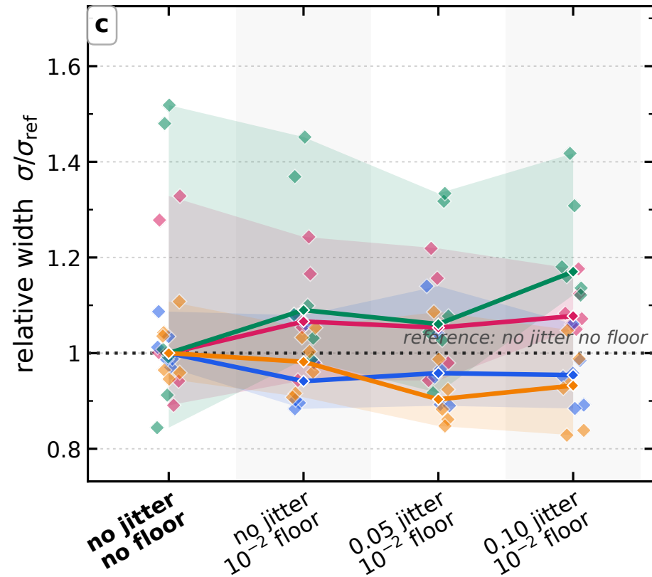
Marginal widths
