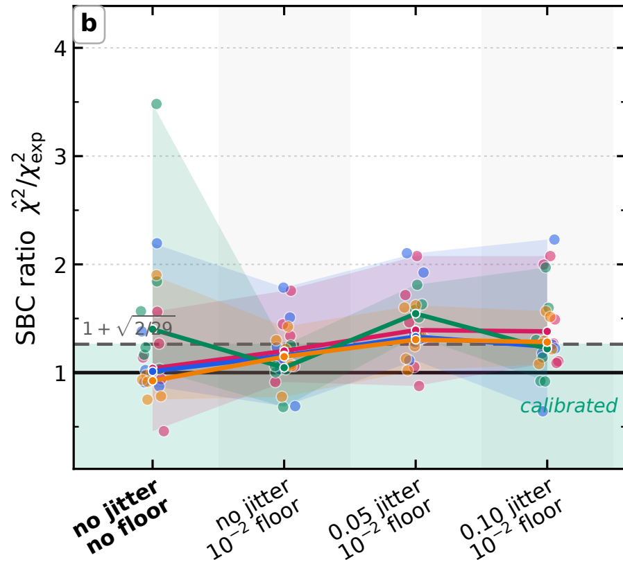
Calibration
