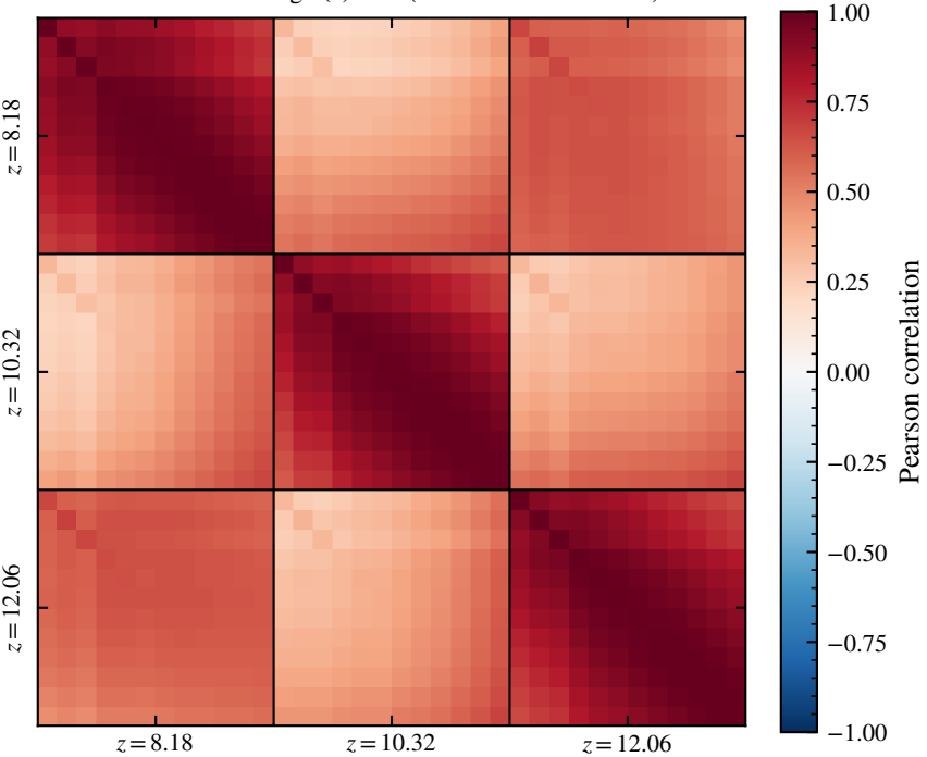
correlation of \log P(k) bins (12 k -bins \times 3 redshifts)
