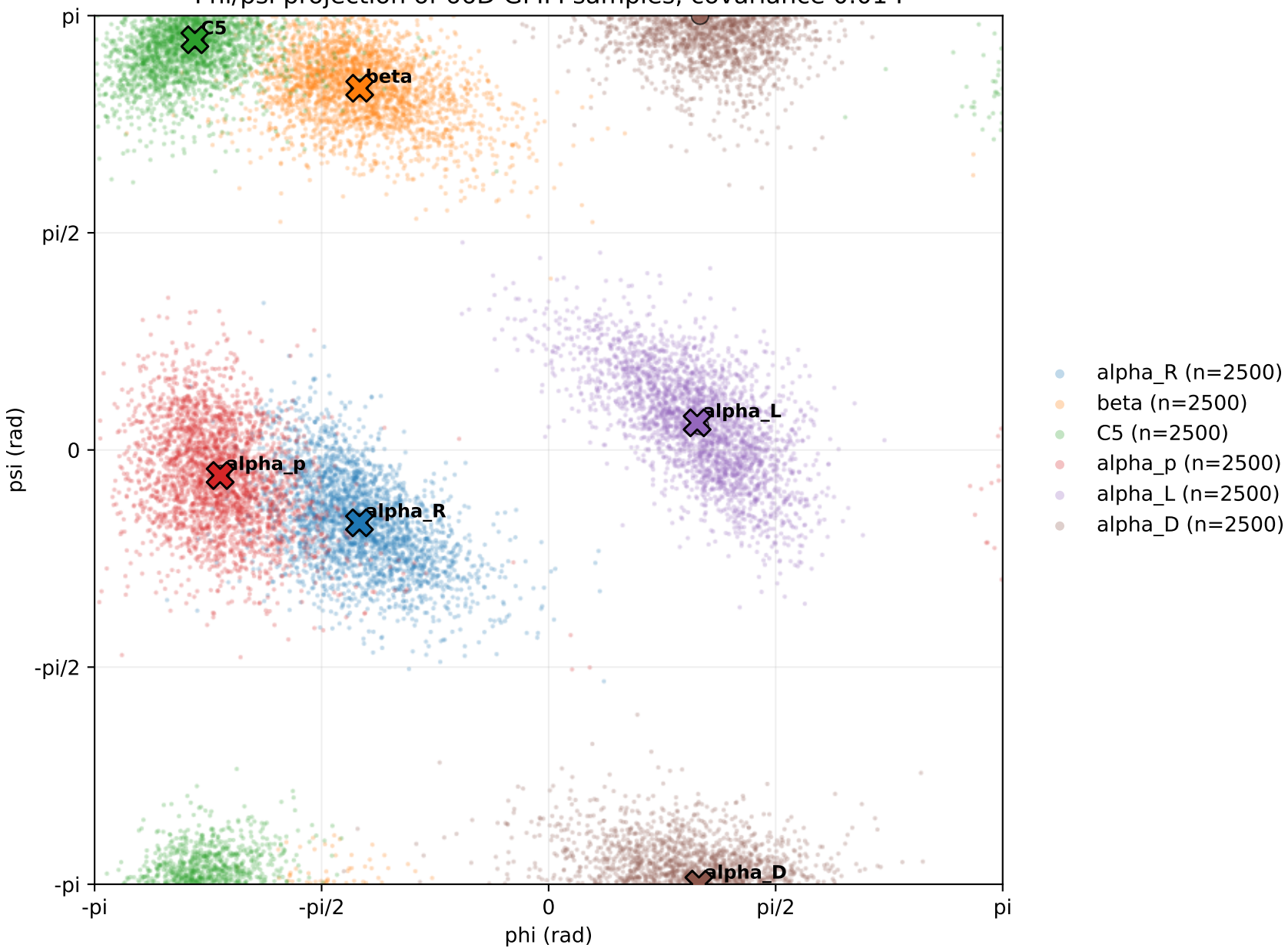
Phi/psi projection of 66D GMM samples, covariance 0.01 I
