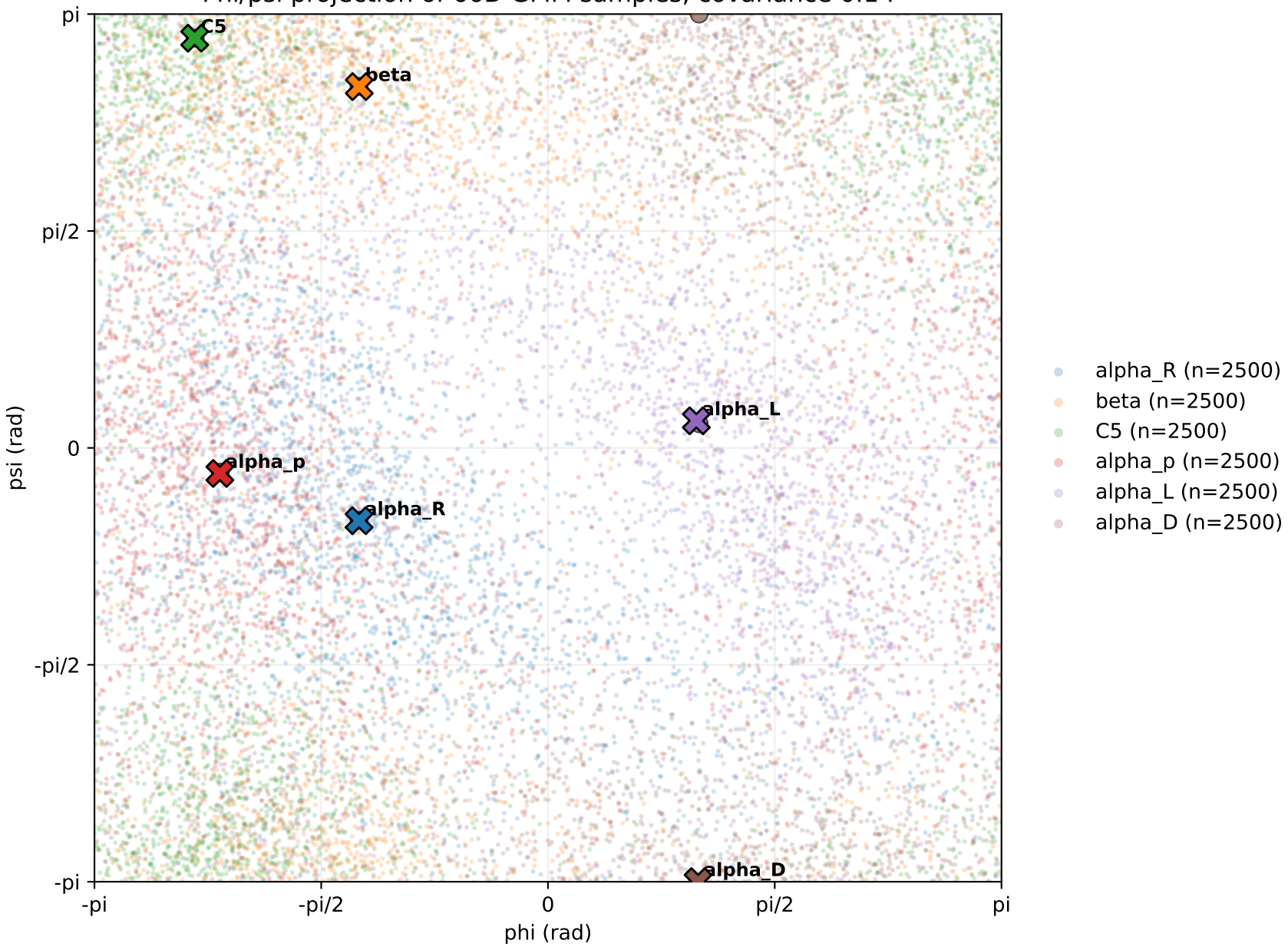
Phi/psi projection of 66D GMM samples, covariance 0.1 I
